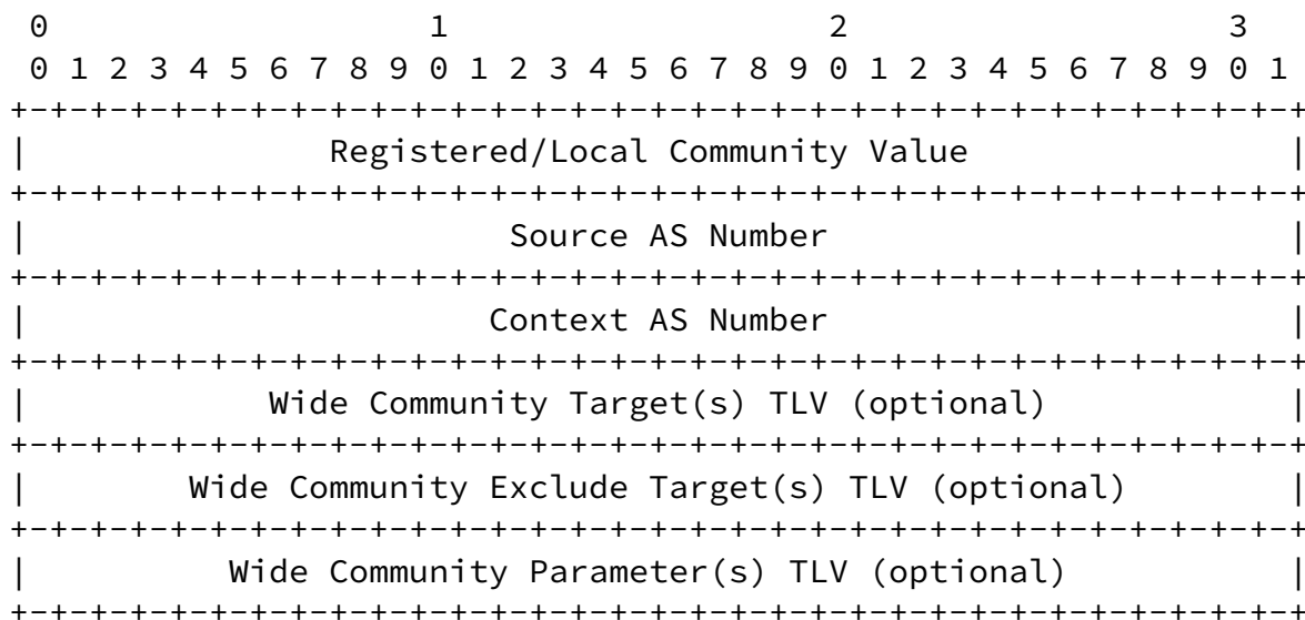
Figure 4: Wide BGP Community Type 1
