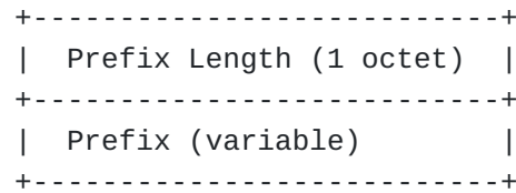
Figure 5: IP prefix atoms
