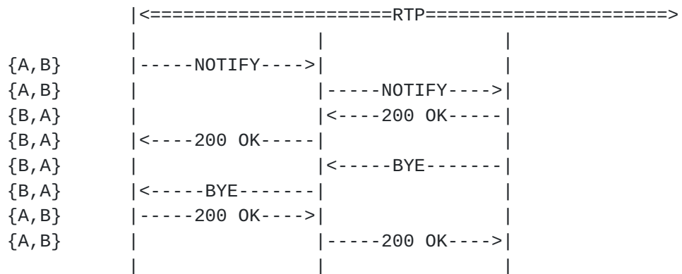
Figure 2 - Call Transfer using REFER
