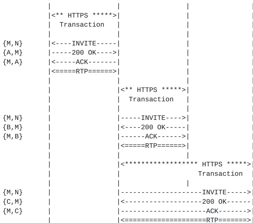
Figure 5 - Single Focus WebEx Conference
