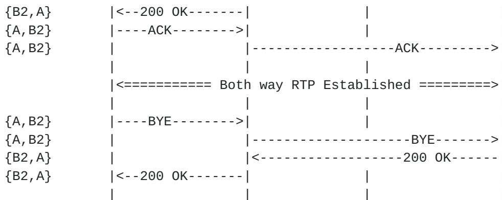
Figure 10 - Session Identifier in the 100 Trying and CANCEL Messaging
