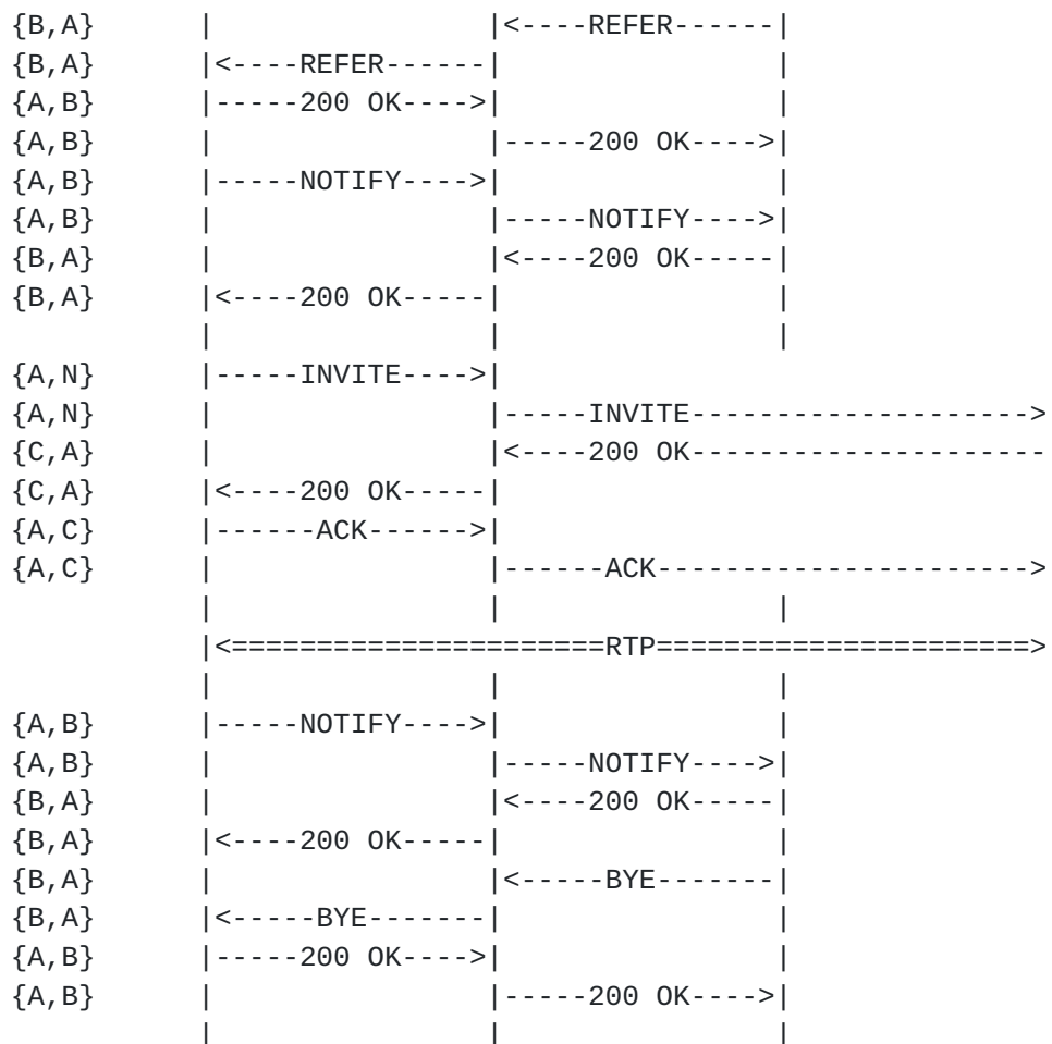
Figure 2 - Call Transfer using REFER
