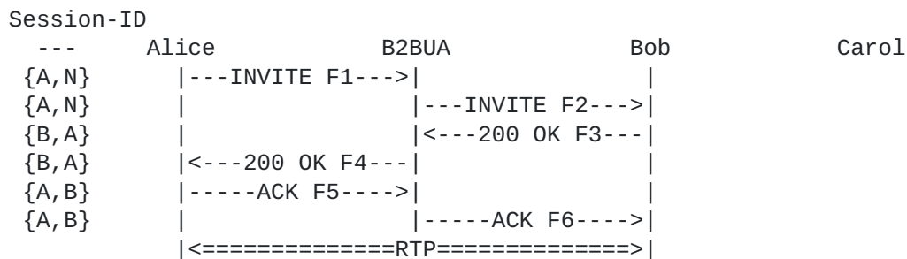
Figure 1: Session-ID Creation when Alice calls Bob
