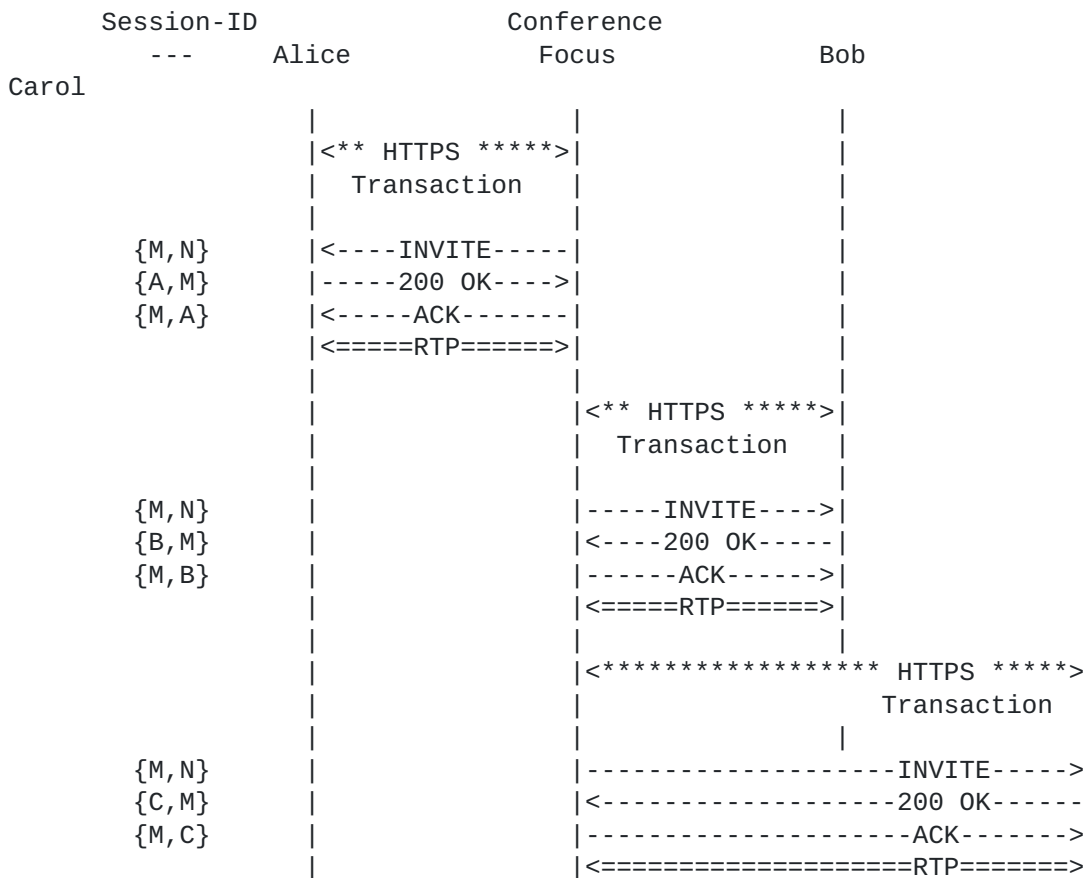
Figure 5: Single Focus Web-based Conference
