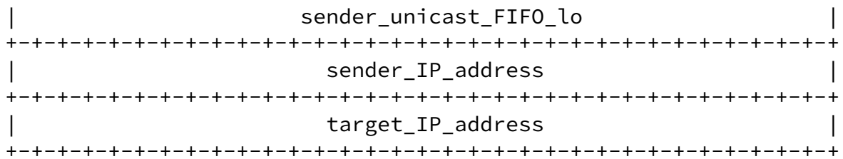
Figure 5 - 1394 ARP request/response format
