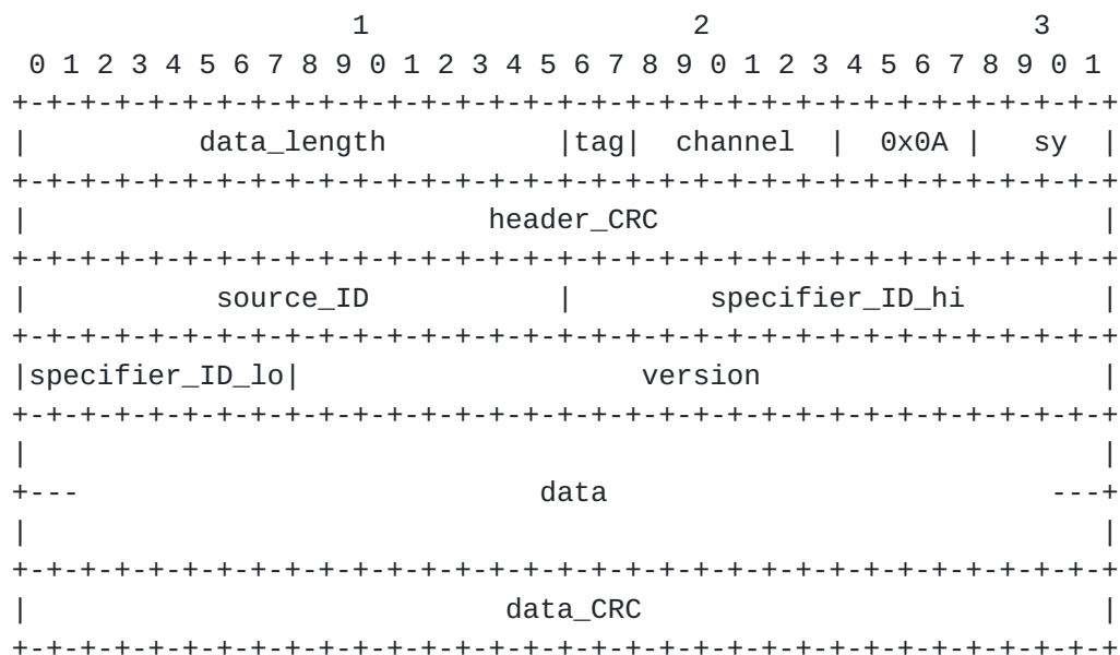
Figure 1 - GASP format
