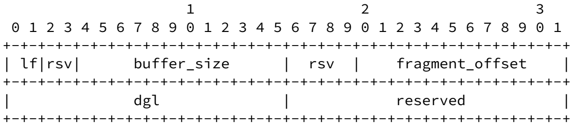
Figure 4 - Subsequent fragment(s) encapsulation header format
