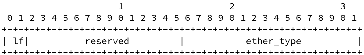
Figure 2 - Unfragmented encapsulation header format
