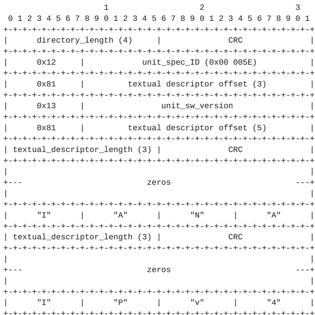
Figure 9 - Sample unit directory and textual descriptors
