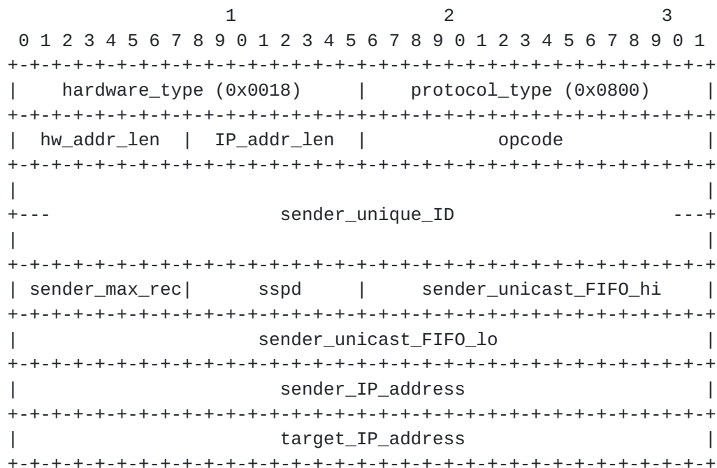
Figure 5 - 1394 ARP request/response format
