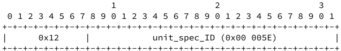
Figure 6 - Unit_Spec_ID entry format
