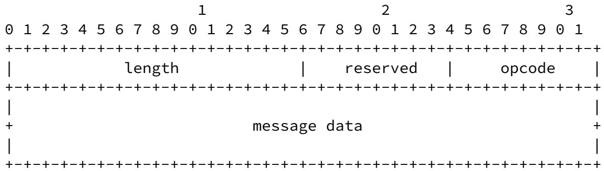
Figure 10 - MCAP message format
