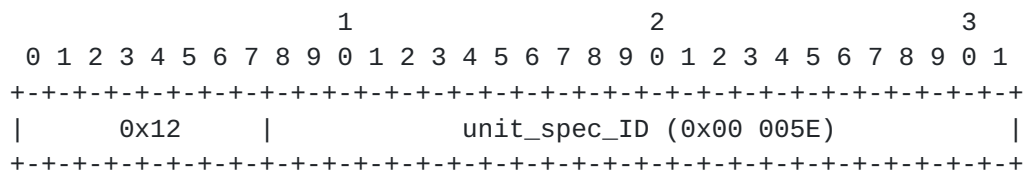
Figure 6 - Unit_Spec_ID entry format
