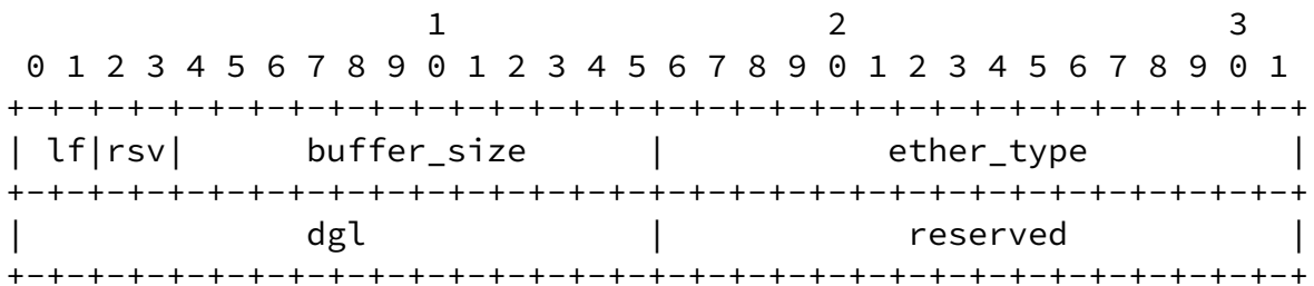
Figure 3 - First fragment encapsulation header format
