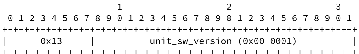
Figure 7 - Unit_SW_Version entry format
