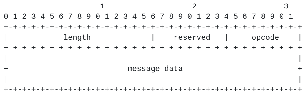
Figure 10 - MCAP message format
