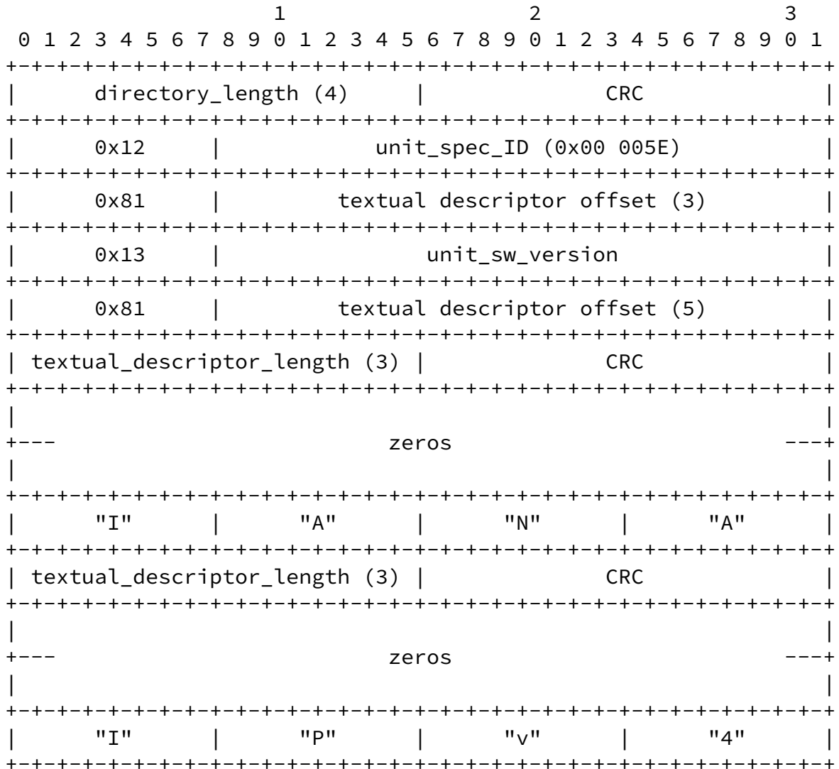
Figure 9 - Sample unit directory and textual descriptors
