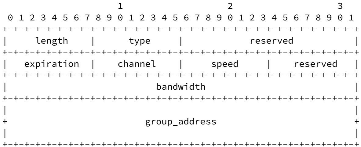
Figure 11 - MCAP group address descriptor format
