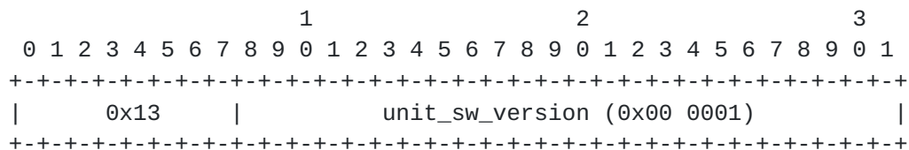
Figure 7 - Unit_SW_Version entry format
