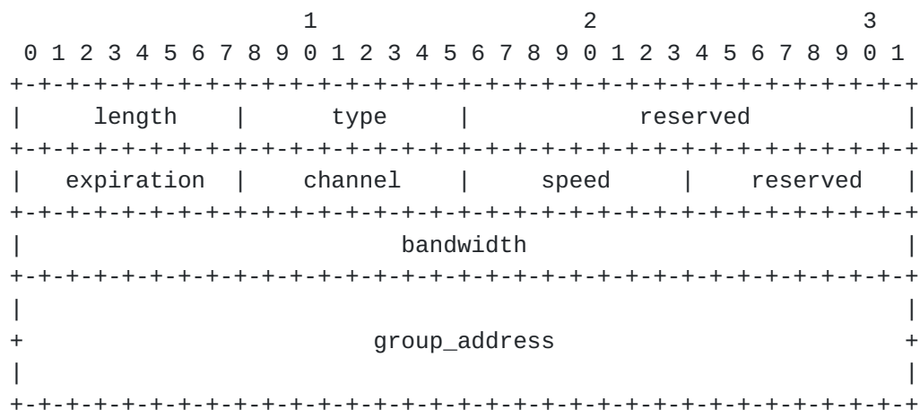
Figure 11 - MCAP group address descriptor format
