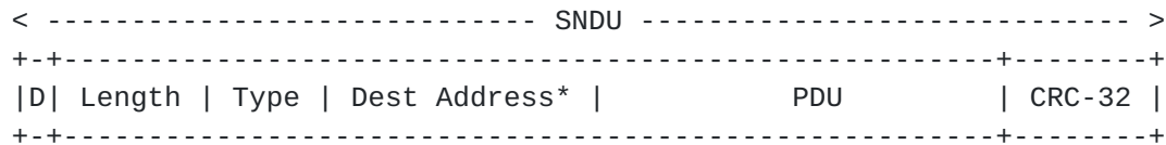
Figure 1: SNDU Encapsulation (* optional Destination Address)
