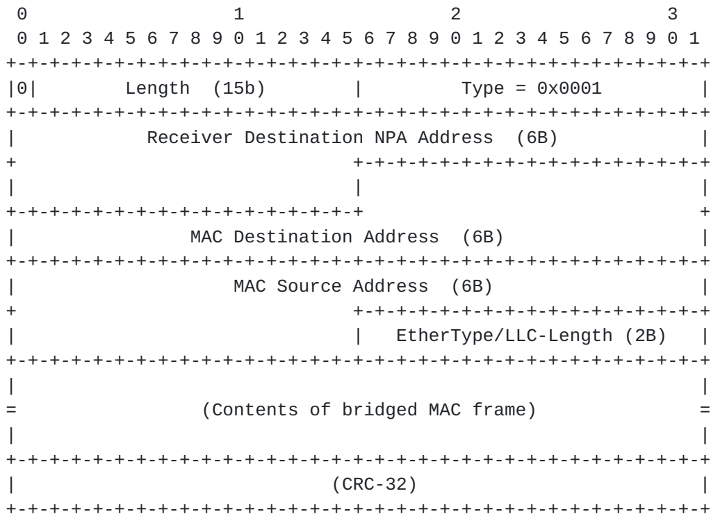
Figure 11: SNDU Format for a Bridged Payload (D=0)
