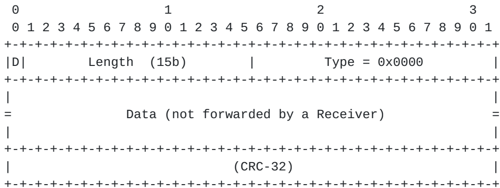
Figure 10: SNDU Format for a Test SNDU
