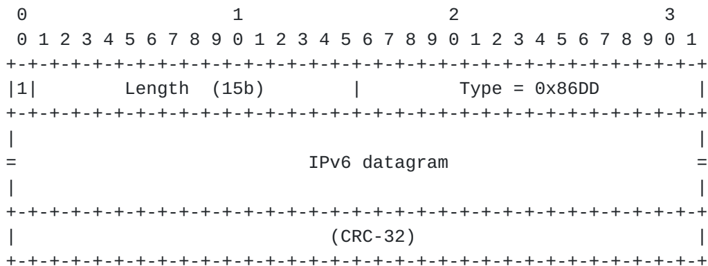
Figure 6: SNDU Format for an IPv6 Datagram using L3 filtering (D=1)
