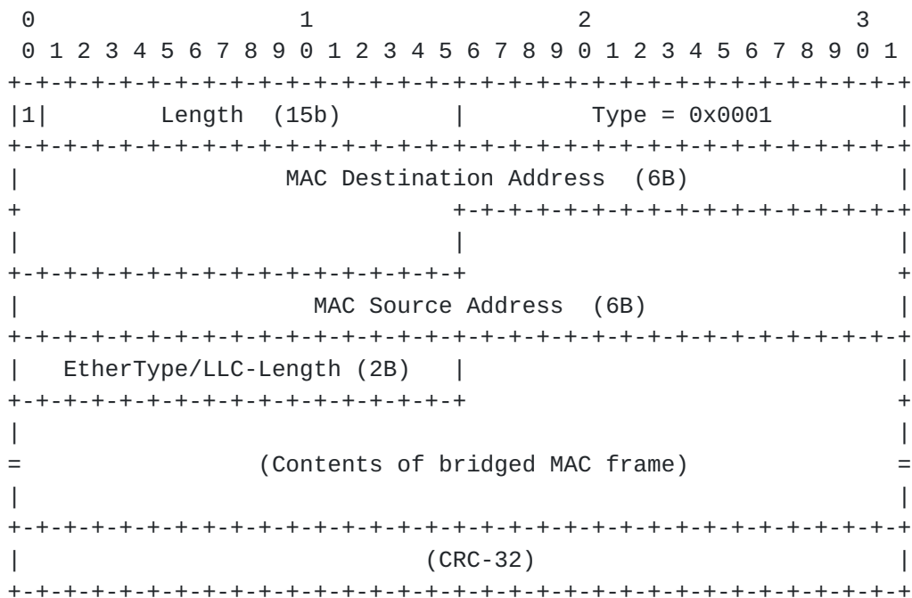
Figure 12: SNDU Format for a Bridged Payload (D=1)
