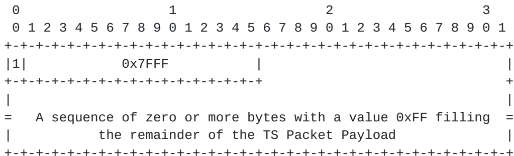
Figure 2: Format for a ULE End Indicator.
