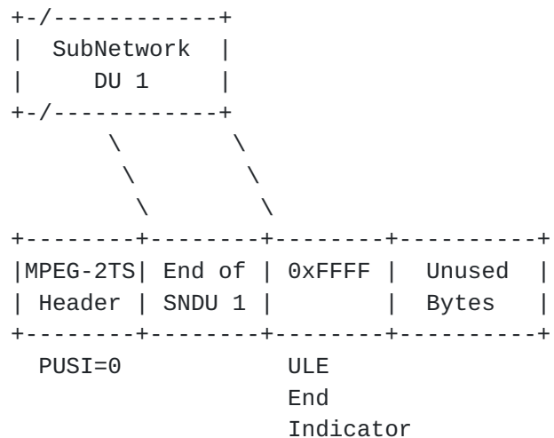
Figure 14: A TS Packet carrying the end of SNDU 1, followed by an End Indicator.
