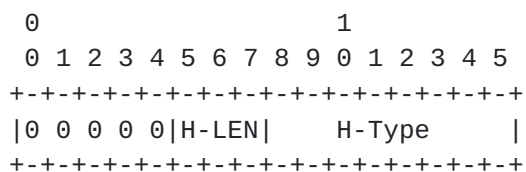
Figure 7: Structure of ULE Next-Header Field.
