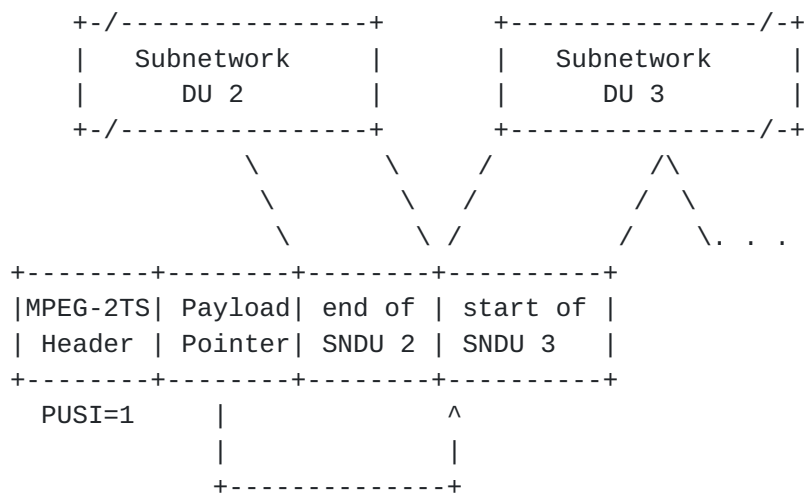
Figure 15: A TS Packet with the end of SNDU 2, followed by SNDU 3.
