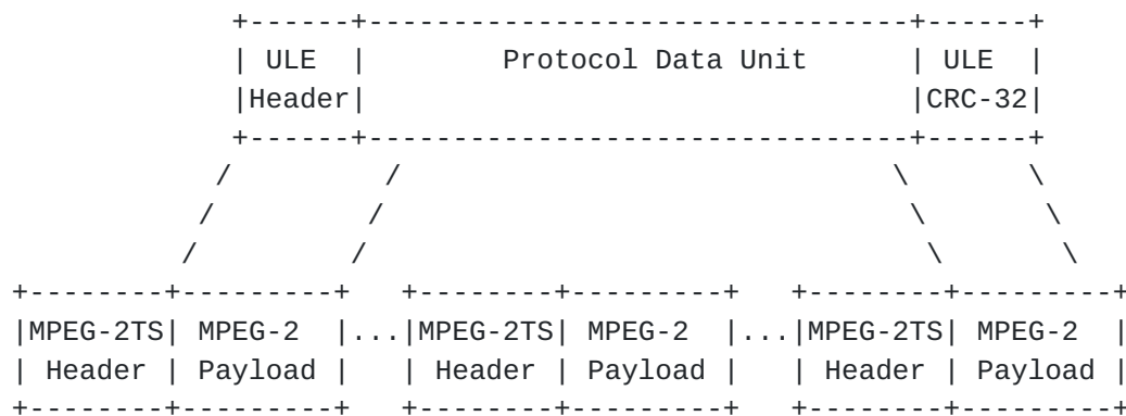
Figure 13: Encapsulation of an SNDU into a series of TS Packets
