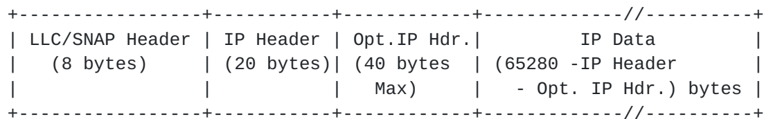
Fig. 4 Format of FC Sequence Payload carrying IP
