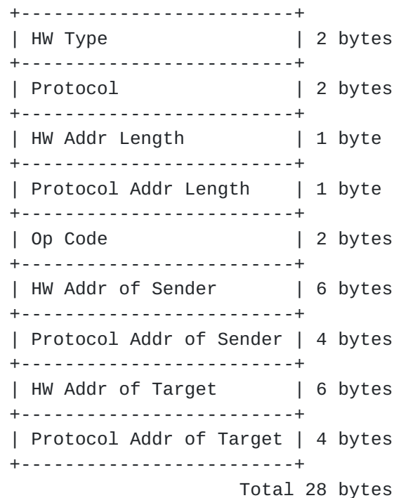
Fig. 9 ARP Packet Format
