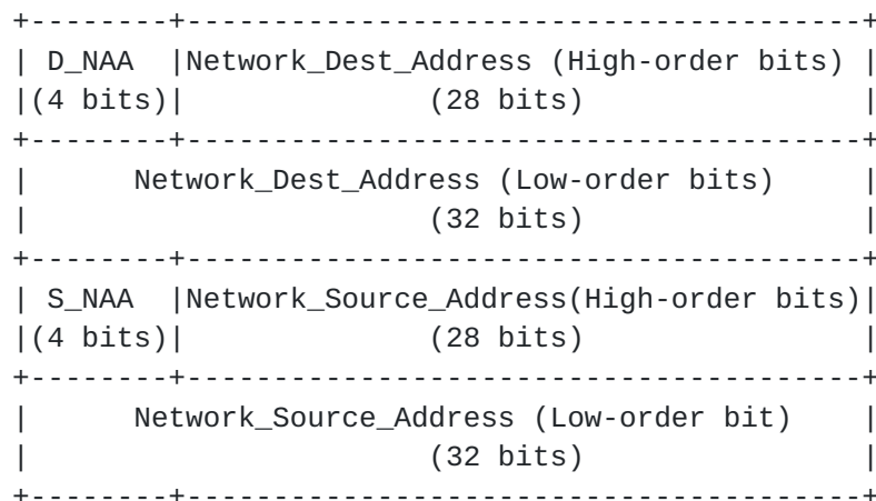
Fig. 3 Format of the Network_Header Field
