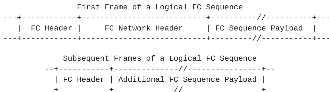
Fig. 2 FC Network_Header in a Frame Sequence
