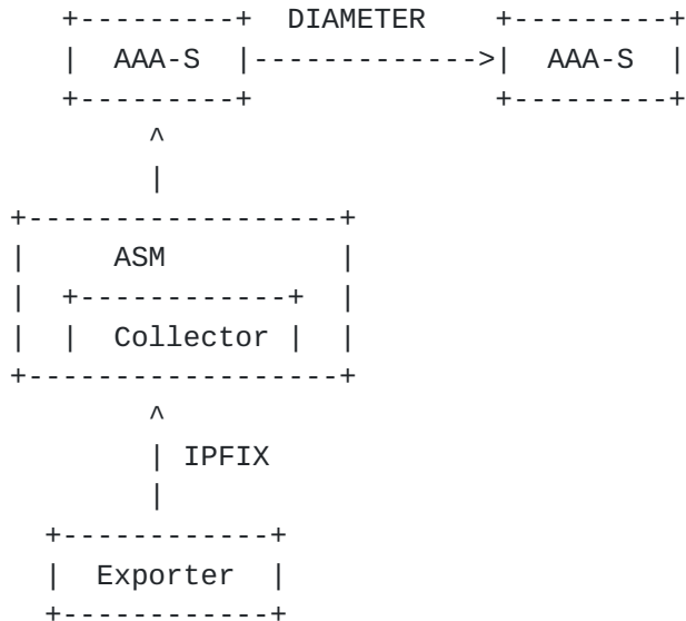
Figure 3: IPFIX connects to AAA server via ASM
