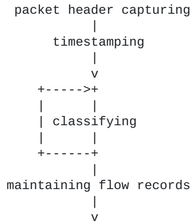
Figure 1: Functions of the metering process
