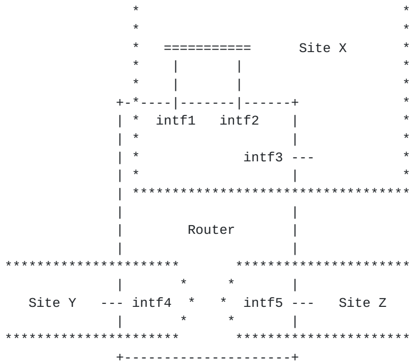
Figure 4: Multi-Sited Router
