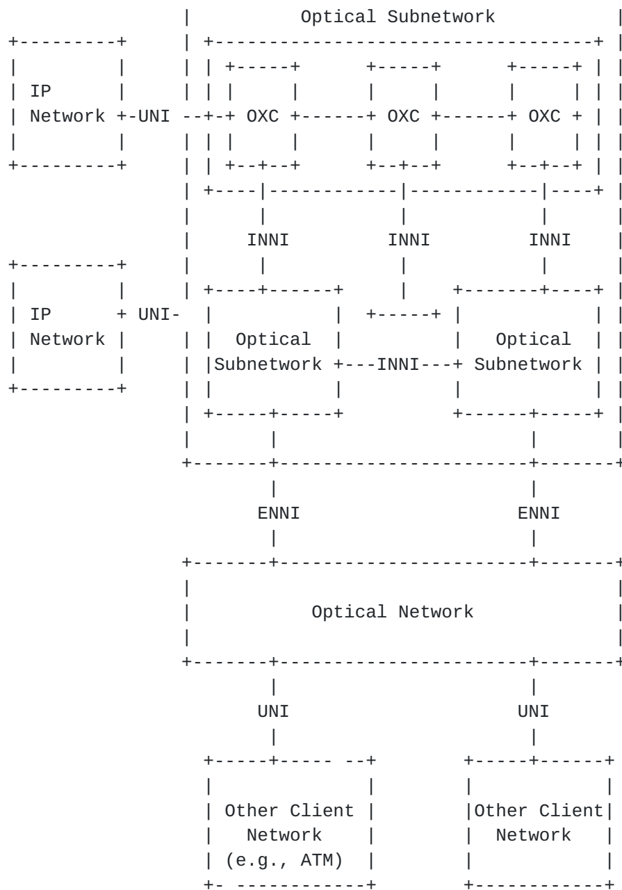
Figure 1: Optical Internetwork Model
