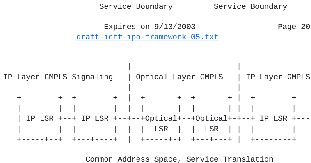
Figure 4: Unified Services Signaling Model
