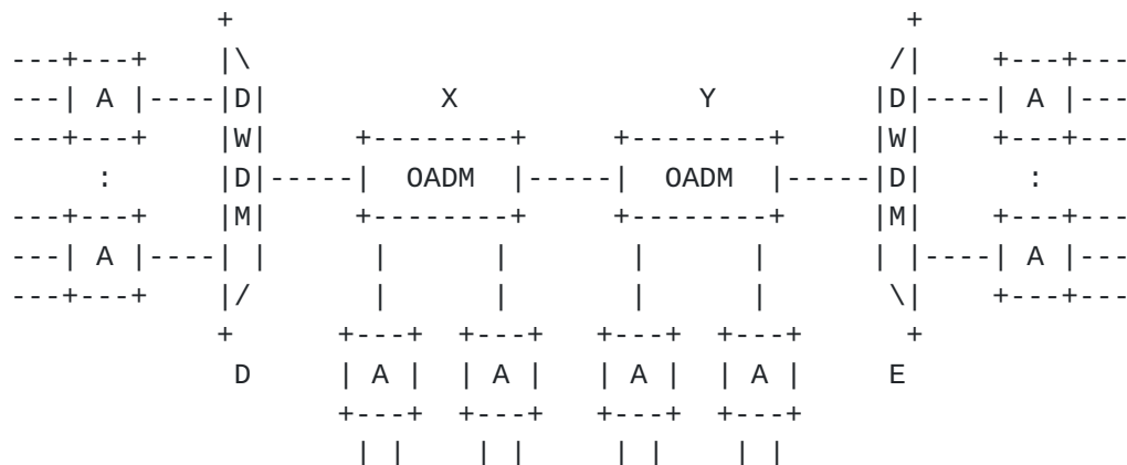
Figure 3-1: An OTS With OADM's - Functional Architecture
