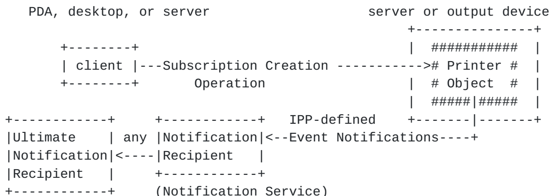
Figure 4 - Use of an Extended Notification Recipient transparent to the Printer
