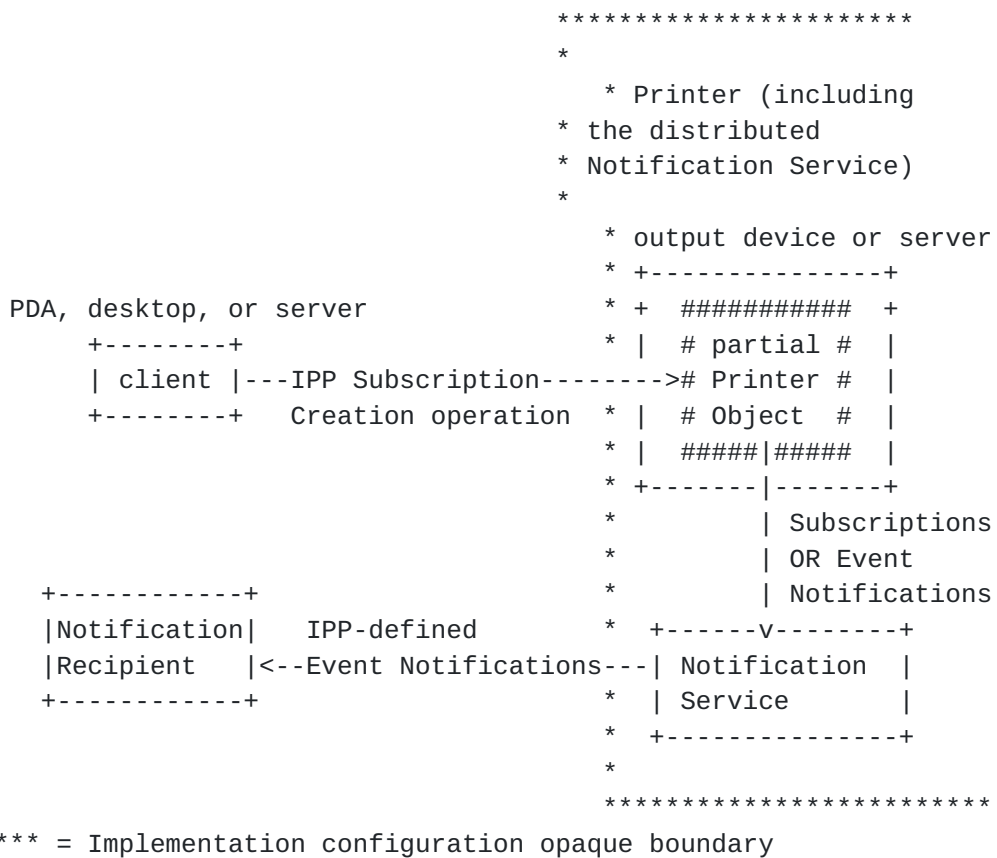
Figure 3 - Opaque Use of a Notification Service Transparent to the Client
