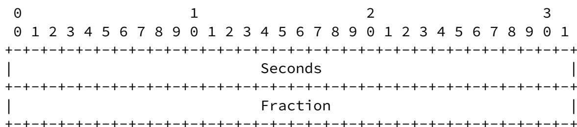
Figure 2: NTP [ RFC5905 ] 64-bit Timestamp Format
