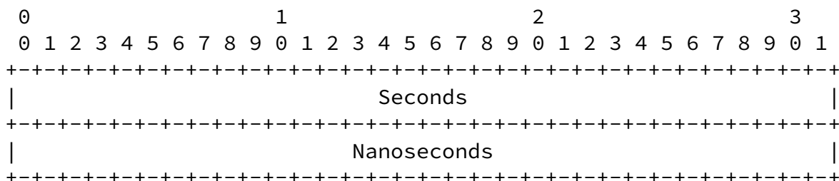
Figure 1: PTP [IEEE1588v2] Truncated Timestamp Format
