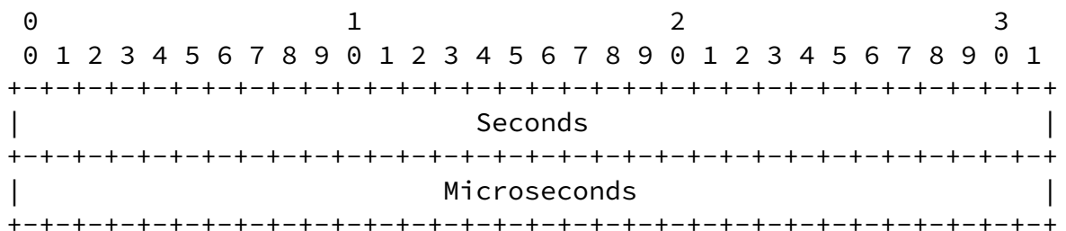
Figure 3: POSIX-based Timestamp Format
