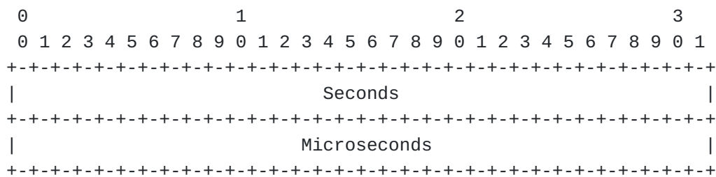
Figure 3: POSIX-based Timestamp Format
