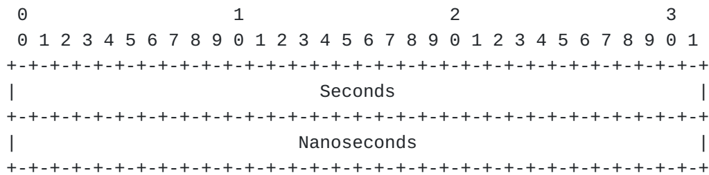
Figure 1: PTP Truncated Timestamp Format
