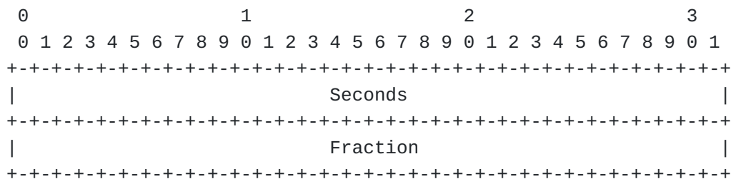
Figure 2: NTP [ RFC5905 ] 64-bit Timestamp Format
