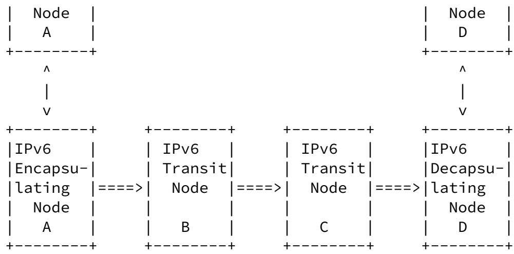
Figure 4: IOAM layering example
