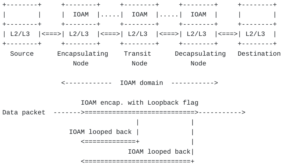
Figure 1: Loopback in IOAM.
