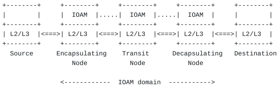
Figure 2: Network using IOAM.
