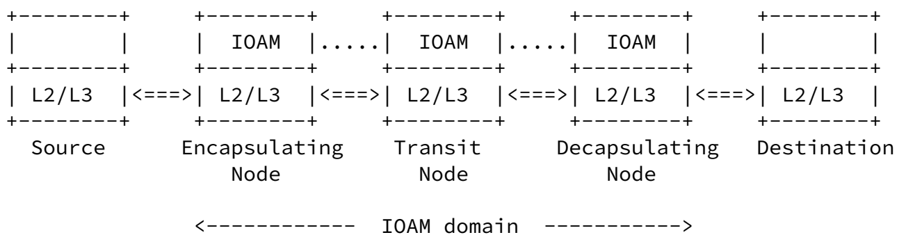
Figure 2: Network using IOAM.
