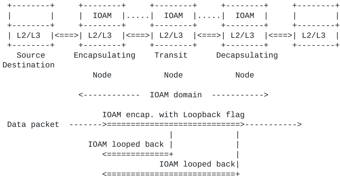
Figure 1: Loopback in IOAM.
