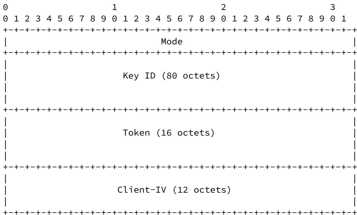
Figure 3: Set-Up-Response Message
