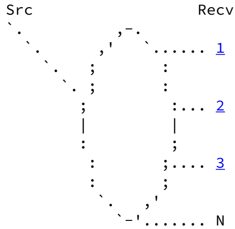
Figure 1: One-to-group points of interest
