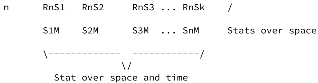
Figure 12: Impact of space aggregation on multimetrics Stat
