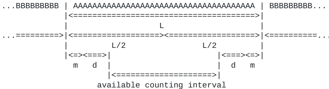
Figure 5: Timing Aspects for Multipoint paths
