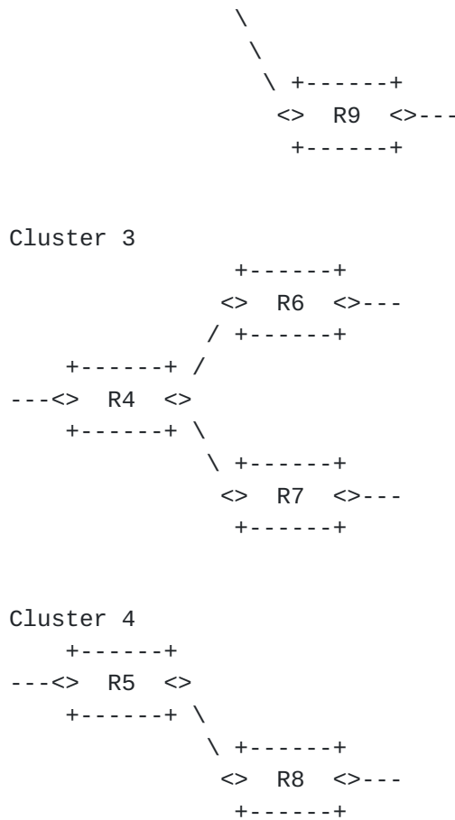
Figure 3: Clusters example
