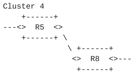
Figure 3: Clusters example
