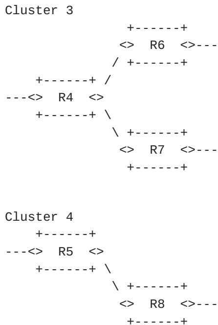
Figure 3: Clusters example
