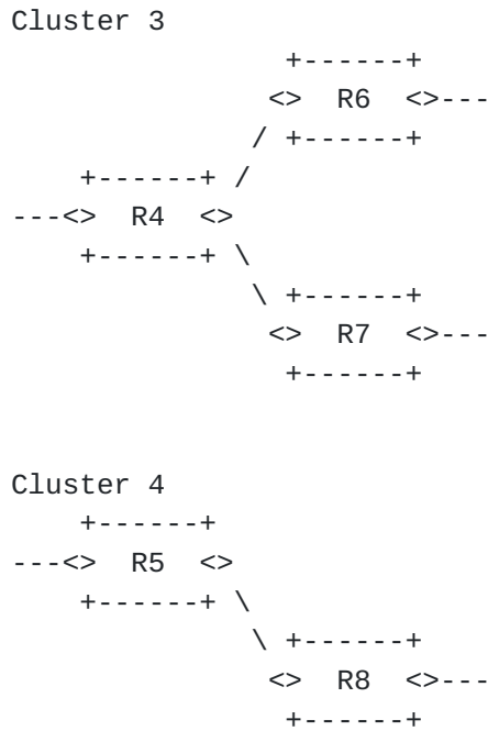
Figure 3: Clusters example
