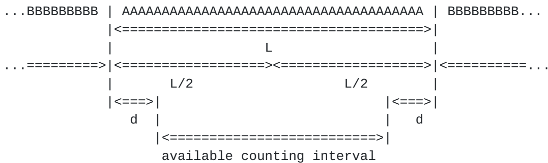
Figure 4: Timing Aspects
