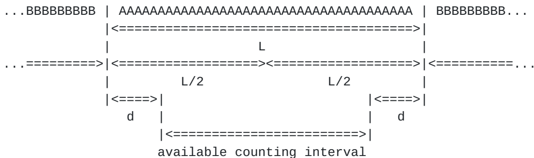
Figure 5: Timing Aspects
