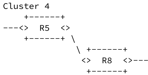
Figure 3: Clusters Example
