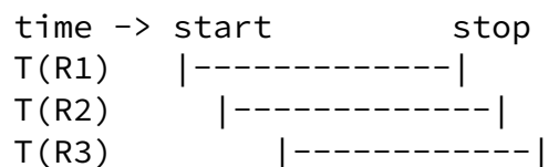
Figure 2: Measurement Interval
