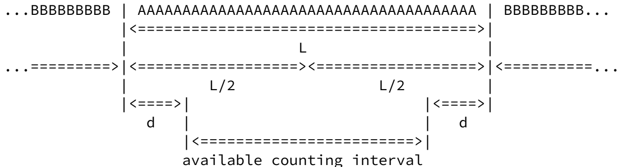
Figure 3: Timing Aspects
