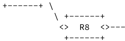
Figure 5: Clusters Example
