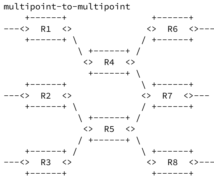
Figure 1: Flow Classification
