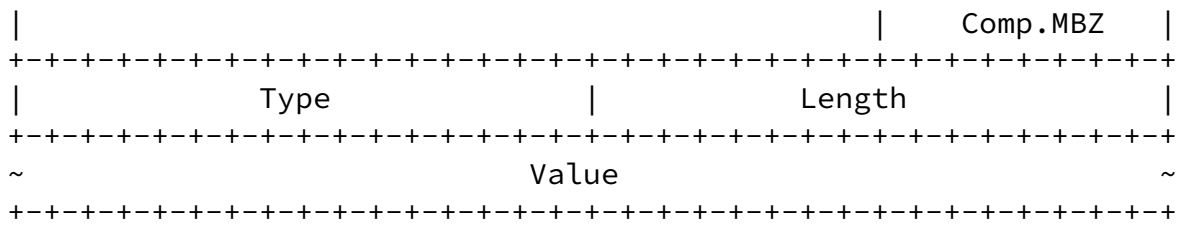
Figure 2: STAMP Session-Sender test packet format in unauthenticated mode
