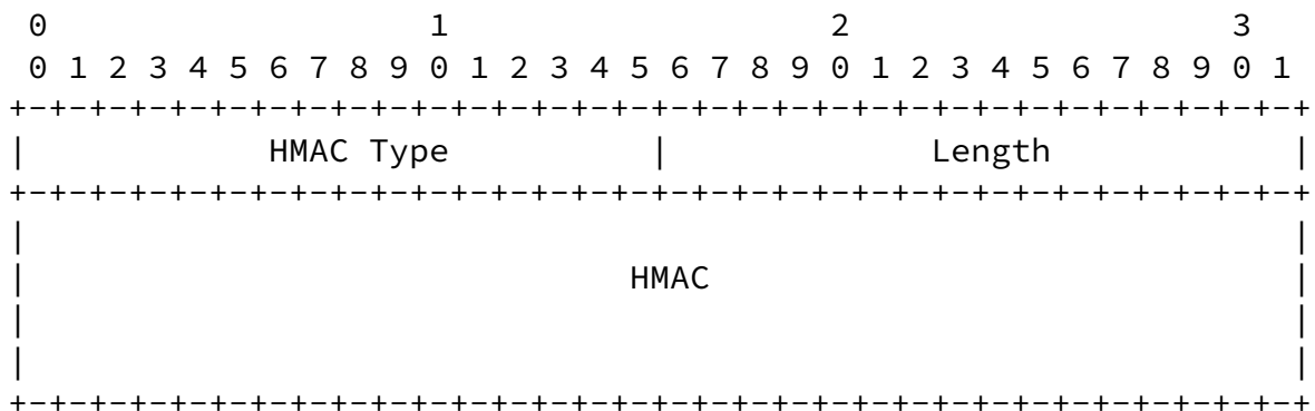
Figure 12: HMAC TLV
