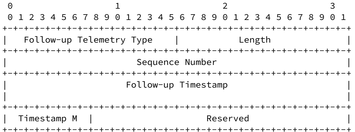
Figure 11: Follow-up Telemetry TLV
