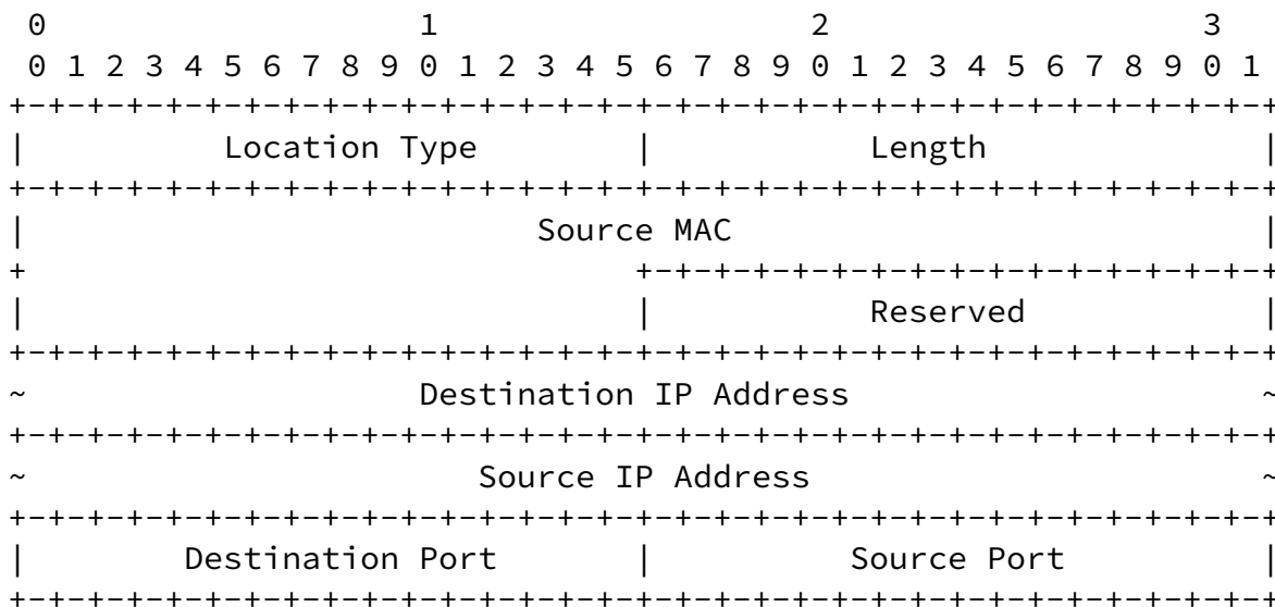
Figure 6: Session-Reflector Location TLV
