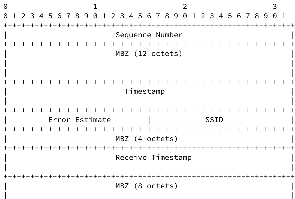
Figure 3: STAMP Session-Sender test packet format in authenticated mode
