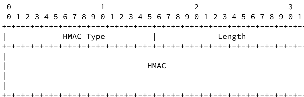
Figure 12: HMAC TLV
