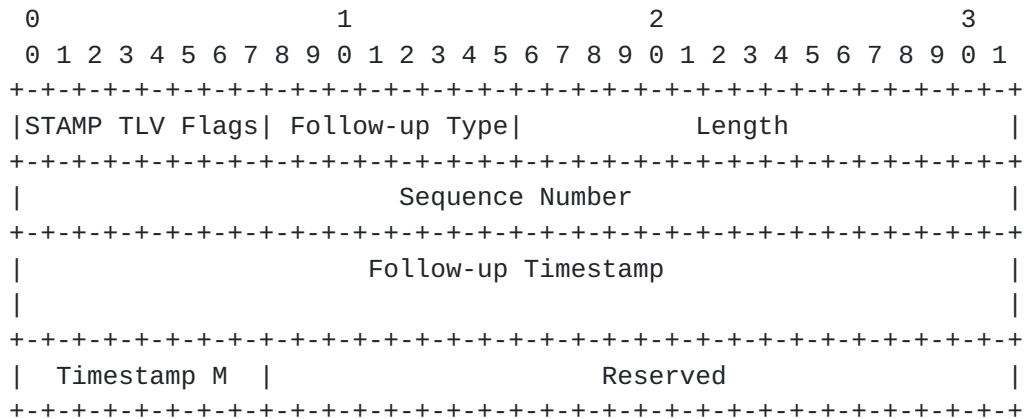
Figure 15: Follow-up Telemetry TLV
