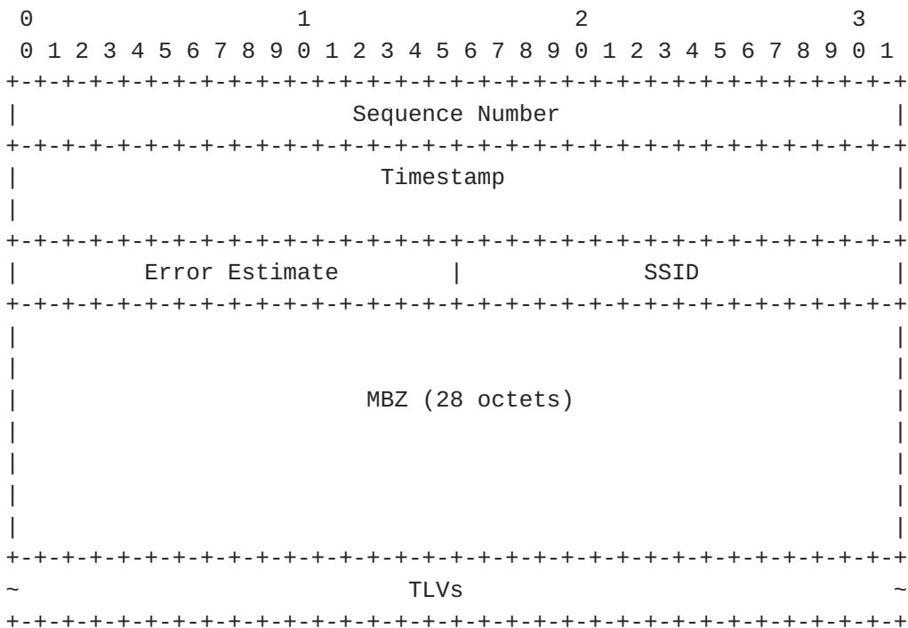
Figure 1: The format of an extended STAMP Session-Sender test packet in unauthenticated mode
