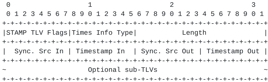
Figure 11: Timestamp Information TLV
