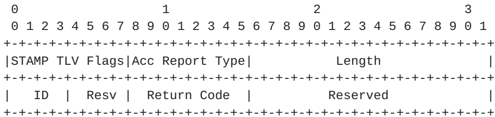
Figure 14: Access Report TLV
