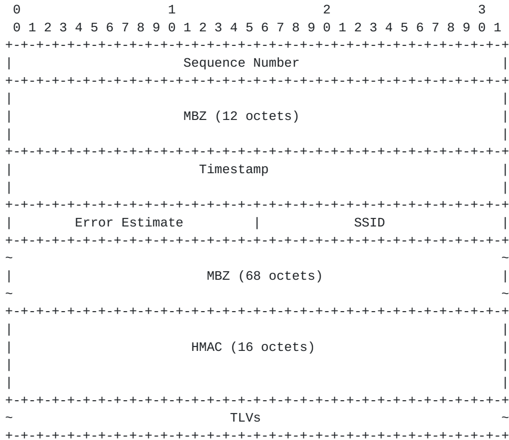
Figure 3: Base STAMP Session-Sender test packet format in authenticated mode
