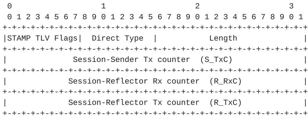
Figure 13: Direct Measurement TLV
