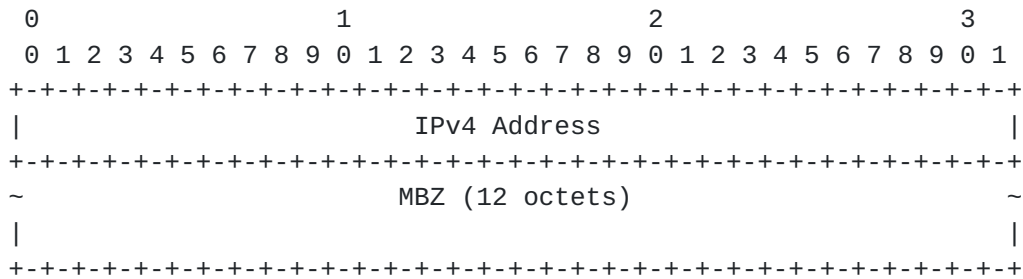
Figure 10: IPv4 Address in a Sub-TLV's Value Field
