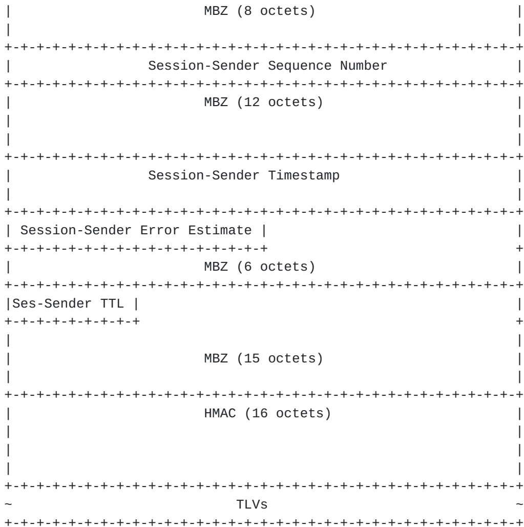
Figure 4: Base STAMP Session-Reflector test packet format in authenticated mode
