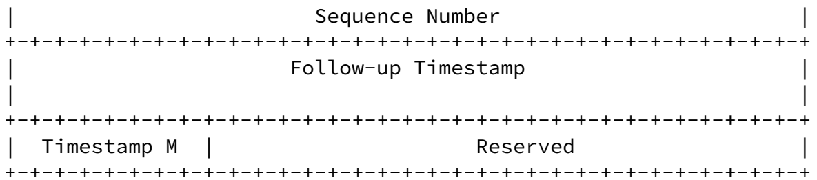
Figure 15: Follow-up Telemetry TLV
