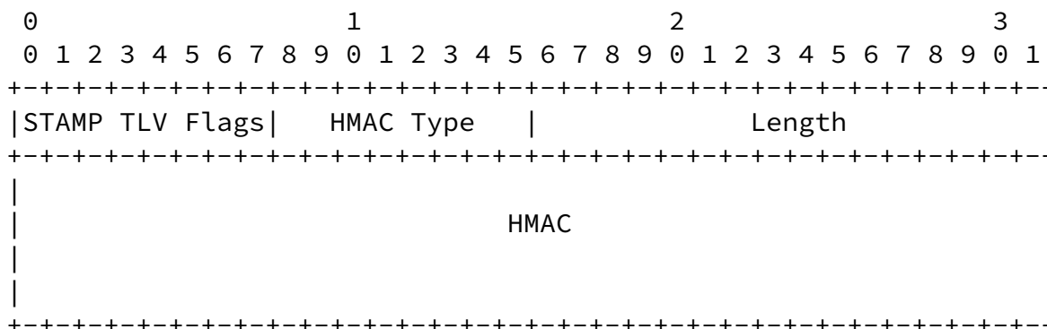
Figure 16: HMAC TLV
