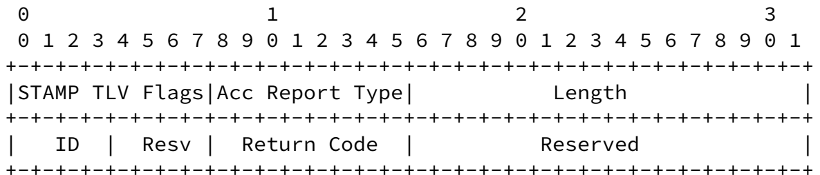
Figure 14: Access Report TLV
