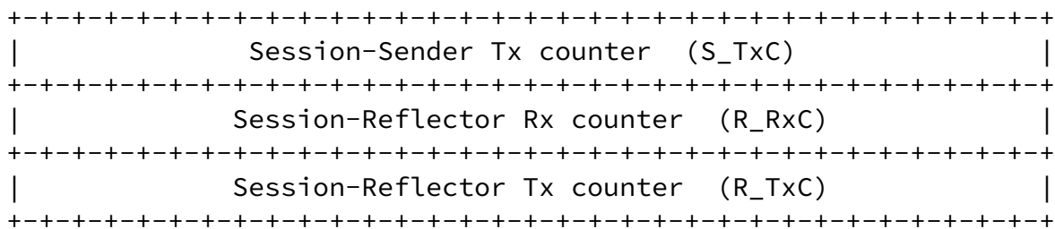
Figure 13: Direct Measurement TLV
