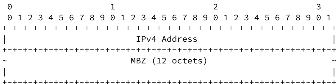
Figure 10: IPv4 Address in a Sub-TLV's Value Field
