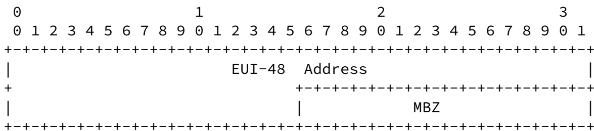
Figure 9: The Value Field of the Source EUI-48 Address sub-TLV
