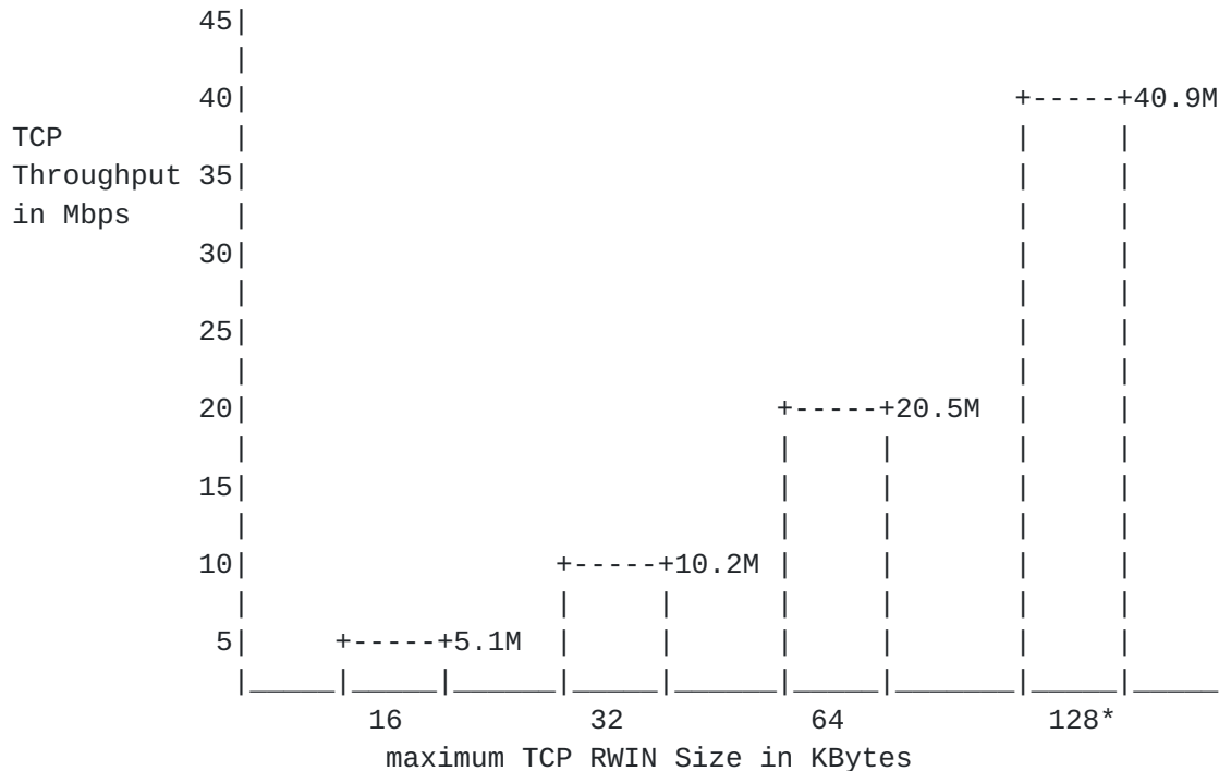
Figure 3.3.1b TCP Throughputs on a T3 with different TCP RWIN
