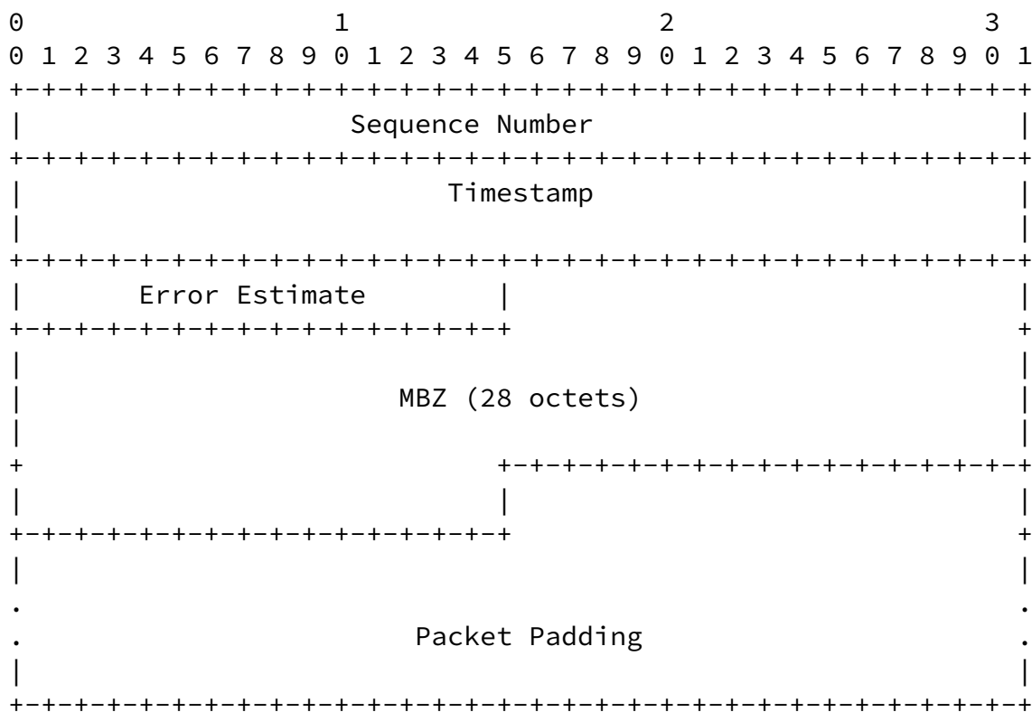
Figure 4: Session-Sender test packet format with DSCP and ECN monitoring and Symmetrical Test Packet in unauthenticated mode
