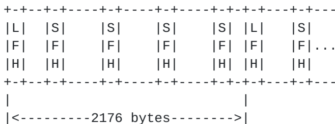
Fig. 14 Example of resynchronization data stream
