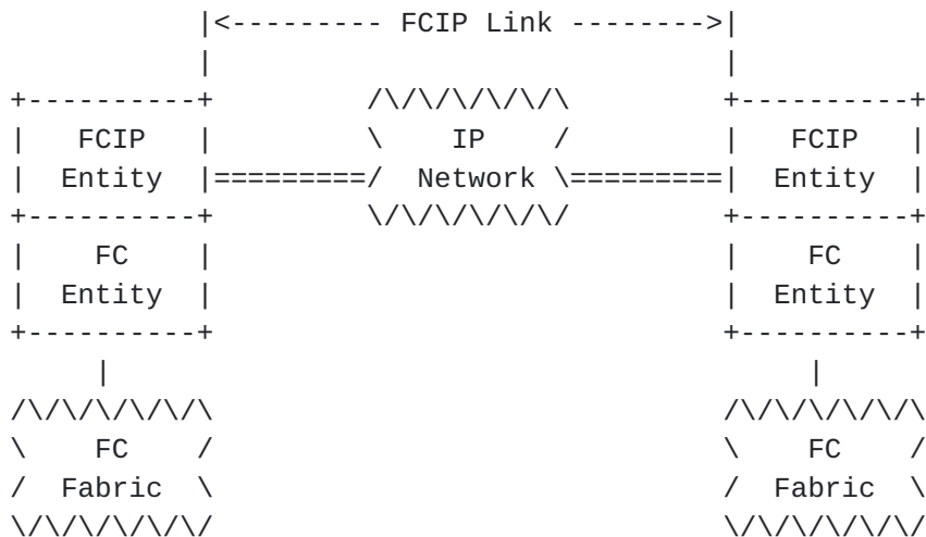
Fig. 3 Model for Two Connected FC/FCIP Entity Pairs
