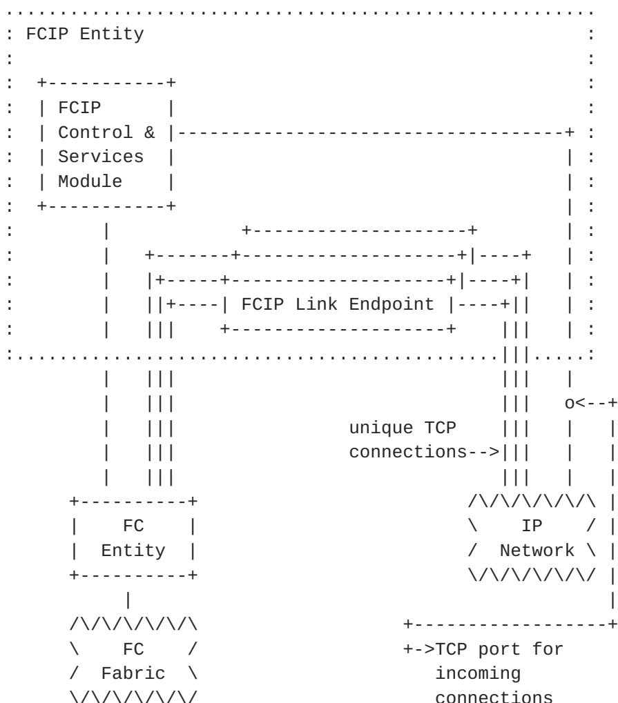
Fig. 4 FCIP Entity Model
