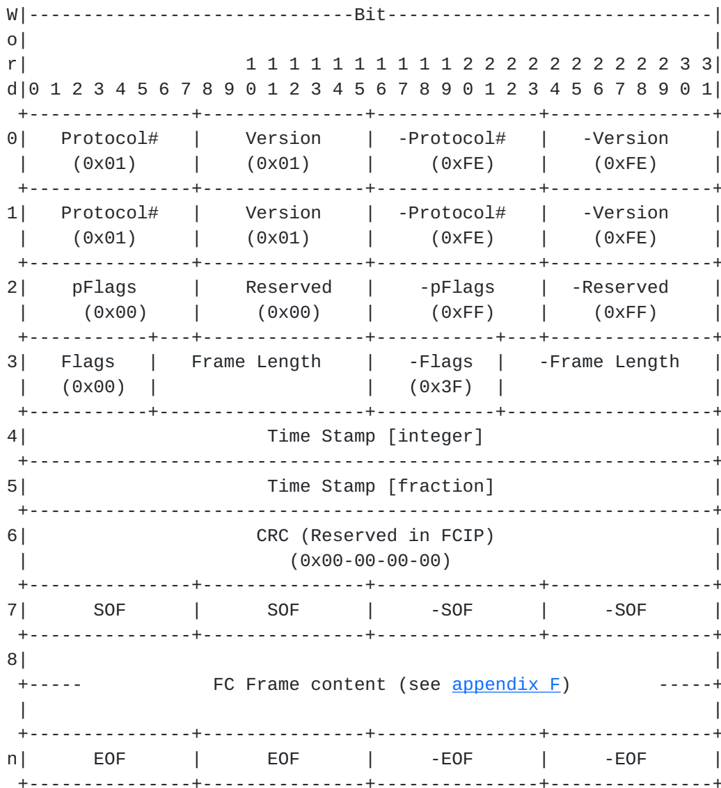
Fig. 17 FCIP Frame Format
