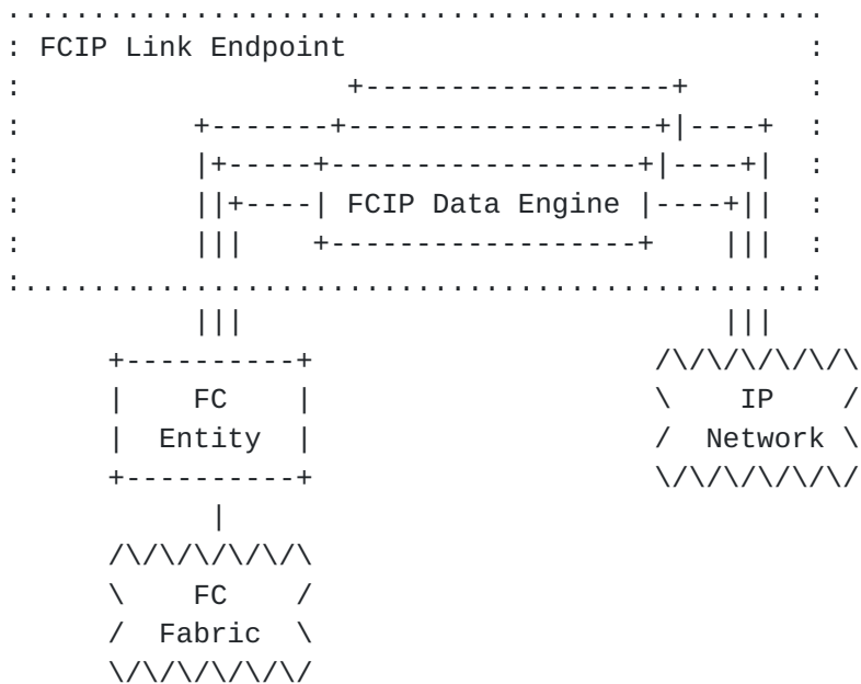
Fig. 5 FCIP Link Endpoint Model
