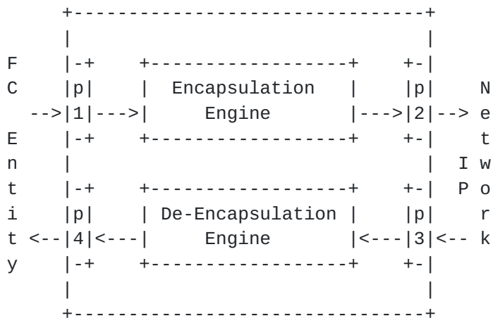
Fig. 6 FCIP Data Engine Model
