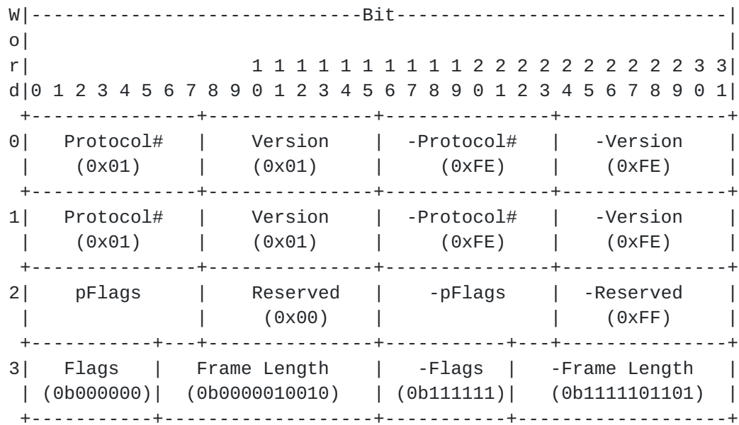
Fig. 9 FSF Format (part 1 of 2)
