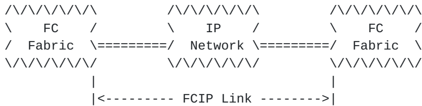
Fig. 2 FCIP Link Model
