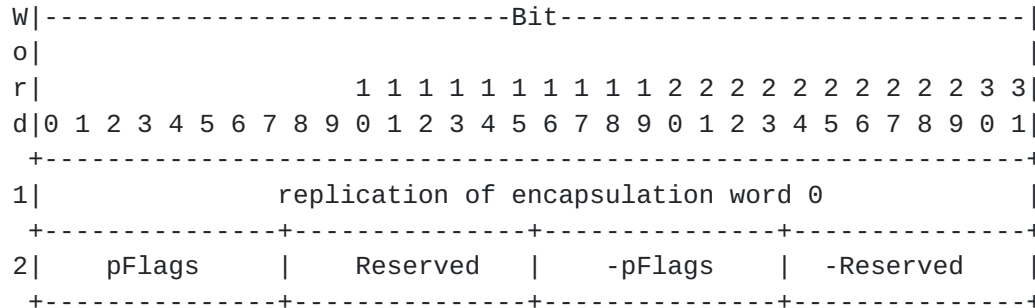
Fig. 7 FCIP Usage of FC Frame Encapsulation Protocol Specific field
