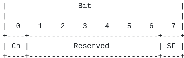
Fig. 8 pFlags Field Bits
