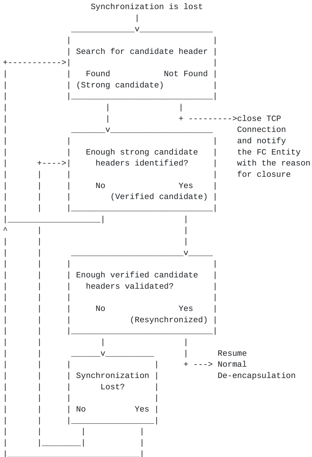
Fig. 15 Flow diagram of simple synchronization example
