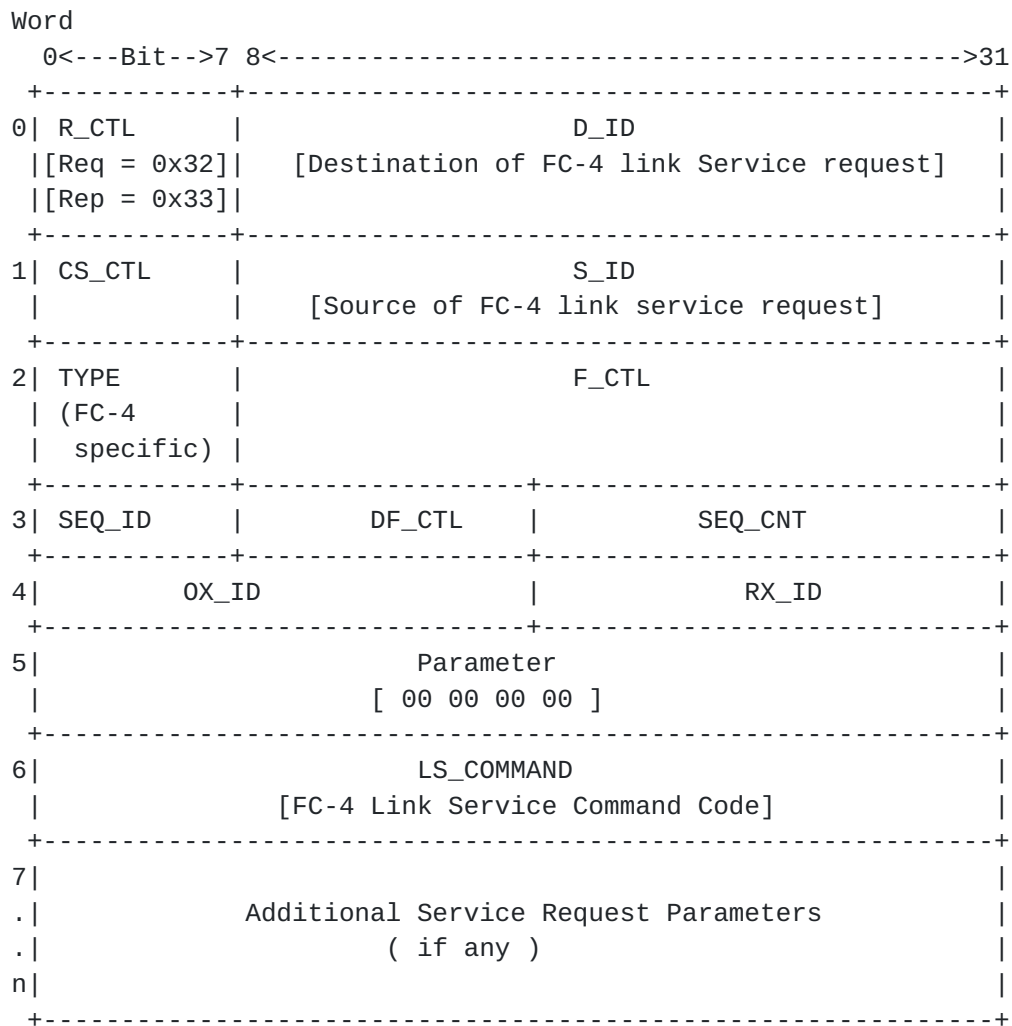
Figure 19 -- Format of an FC-4 Link Service Frame
