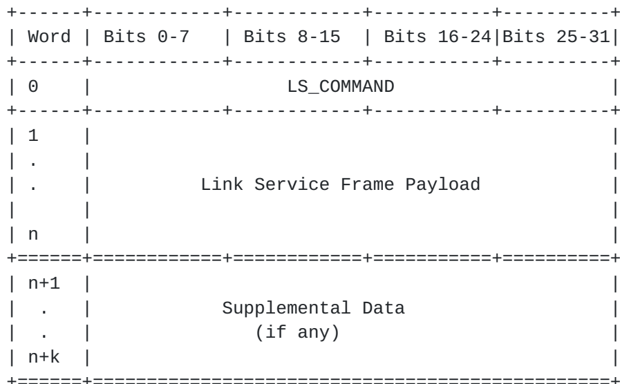
Figure 20 -- Special Link Service Frame Payload
