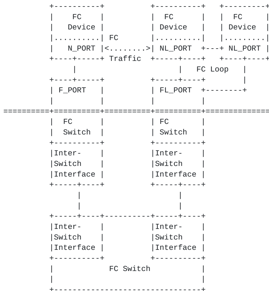
Figure 3 -- Mixed Fibre Channel Fabric
