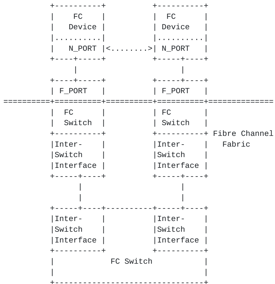
Figure 2 -- Multi-Switch Fibre Channel Fabric
