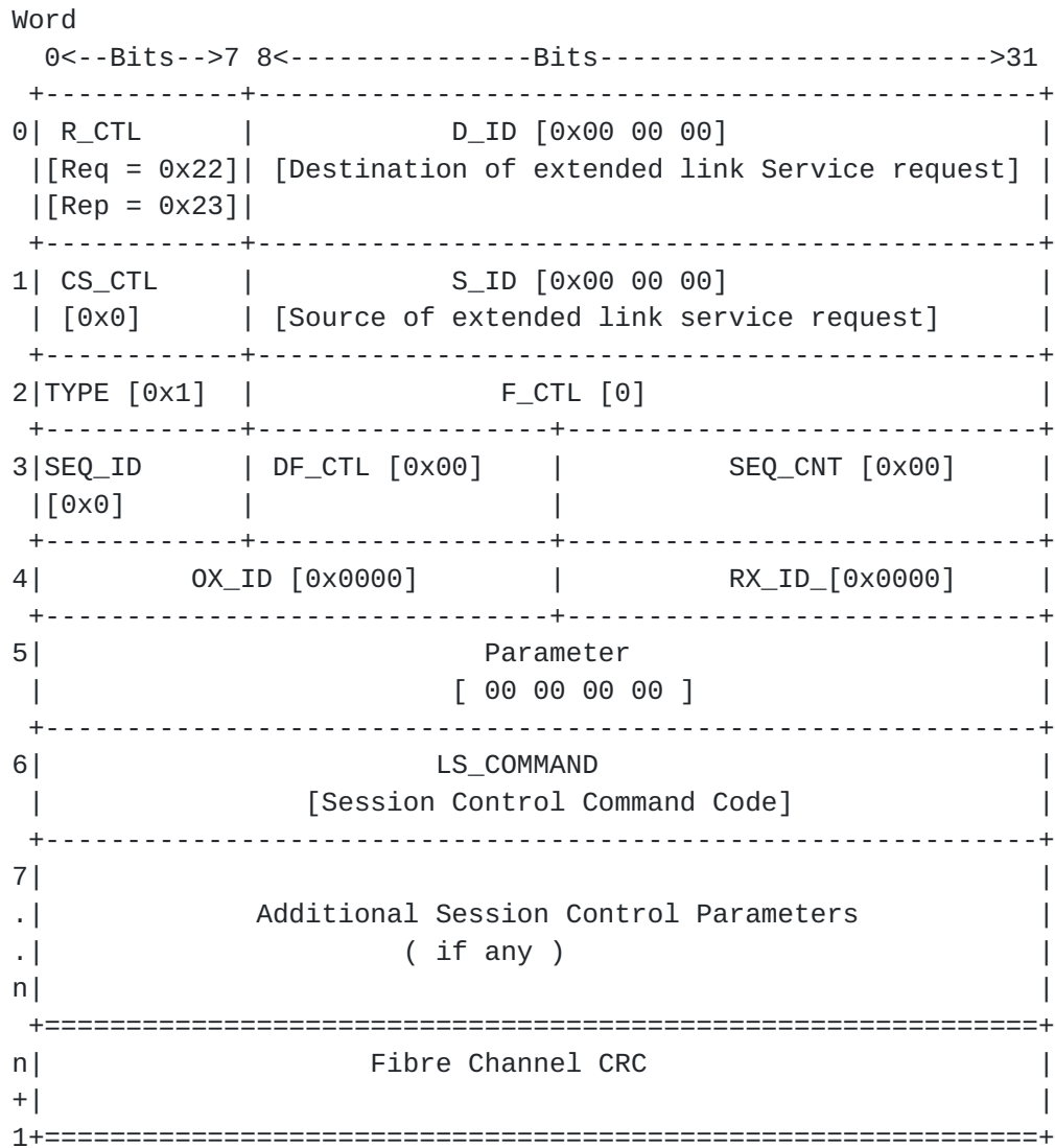
Figure 17 -- Format of Session Control Message
