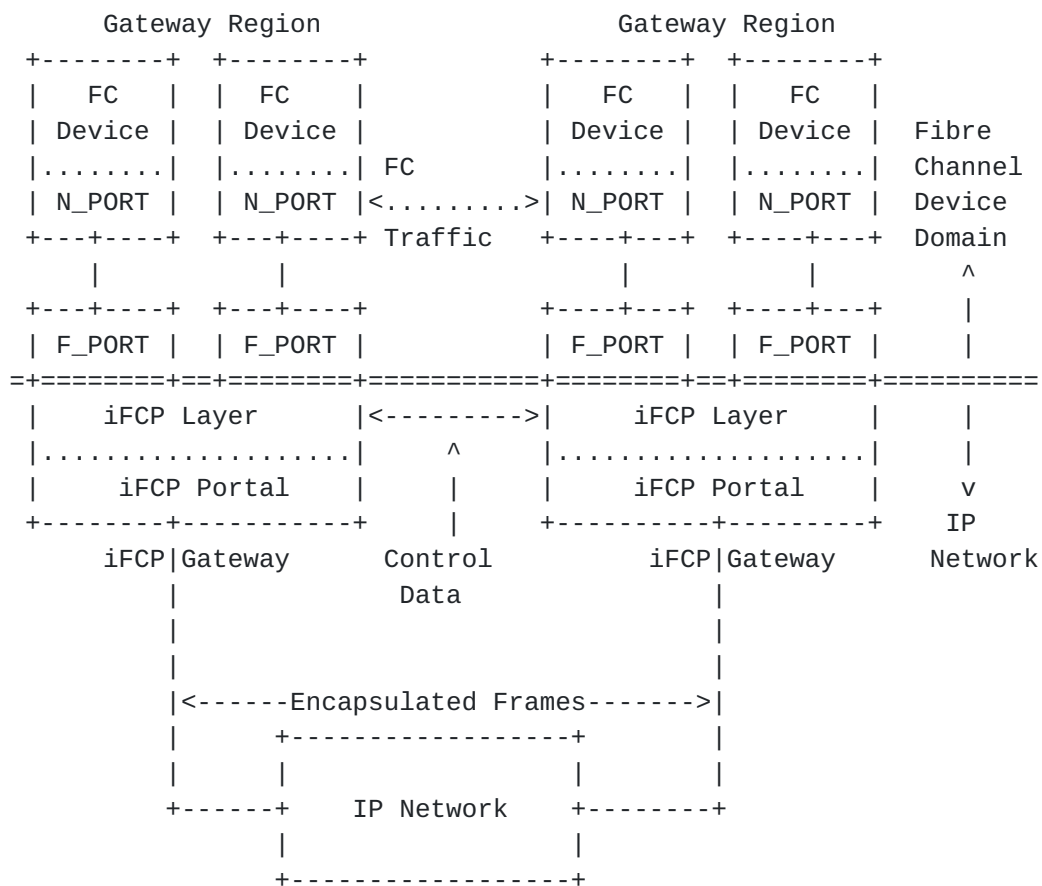
Figure 7 -- An iFCP Fabric Example
