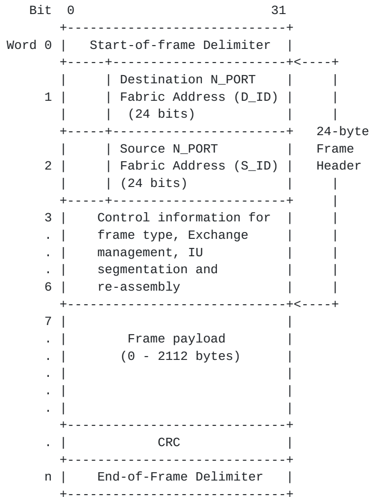
Figure 4 -- Fibre Channel Frame Format
