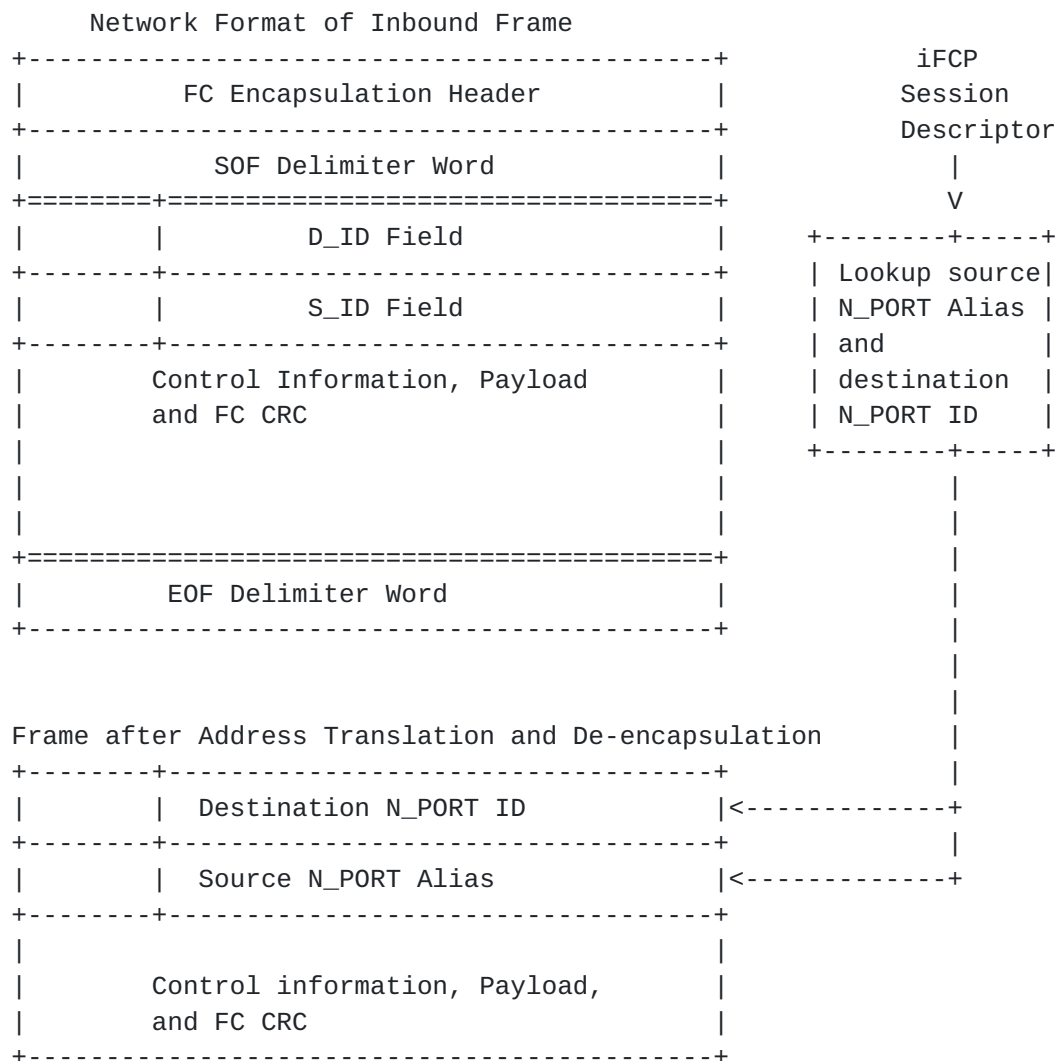
Figure 9 -- Inbound Frame Address Translation
