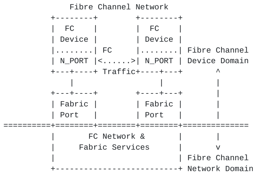
Figure 6 -- A Fibre Channel Network
