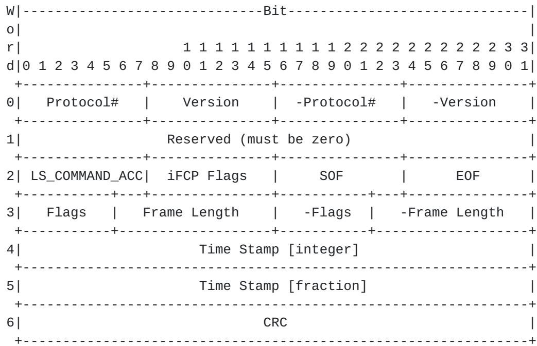
Figure 13 --- Encapsulation Header Format
