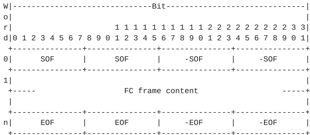
Figure 16 -- FC Frame Encapsulation Format
