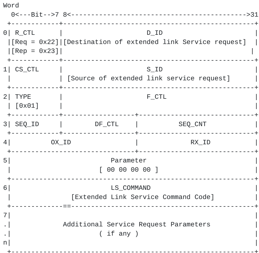
Figure 18 -- Format of an Extended Link Service Frame
