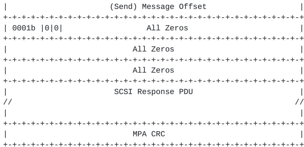
Figure 13 SendInvSE Message containing SCSI Response PDU
