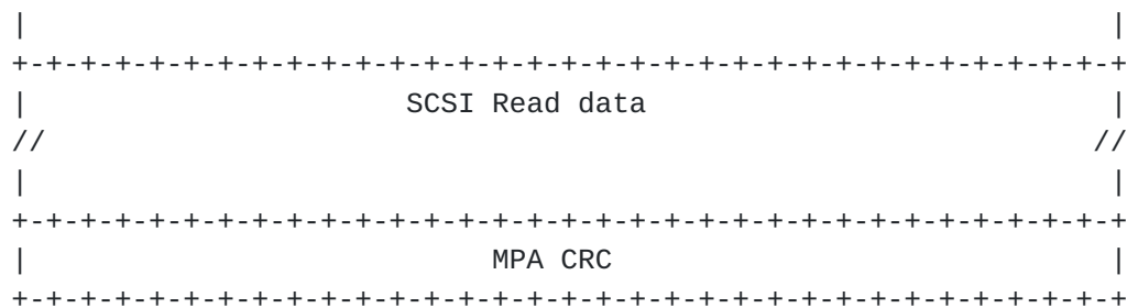
Figure 9 RDMA Write Message containing SCSI Read Data
