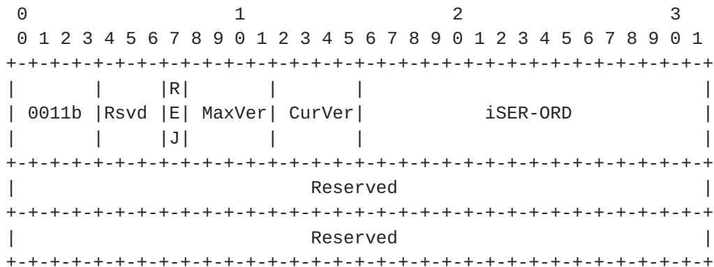
Figure 5 iSER Header Format for iSER HelloReply Message
