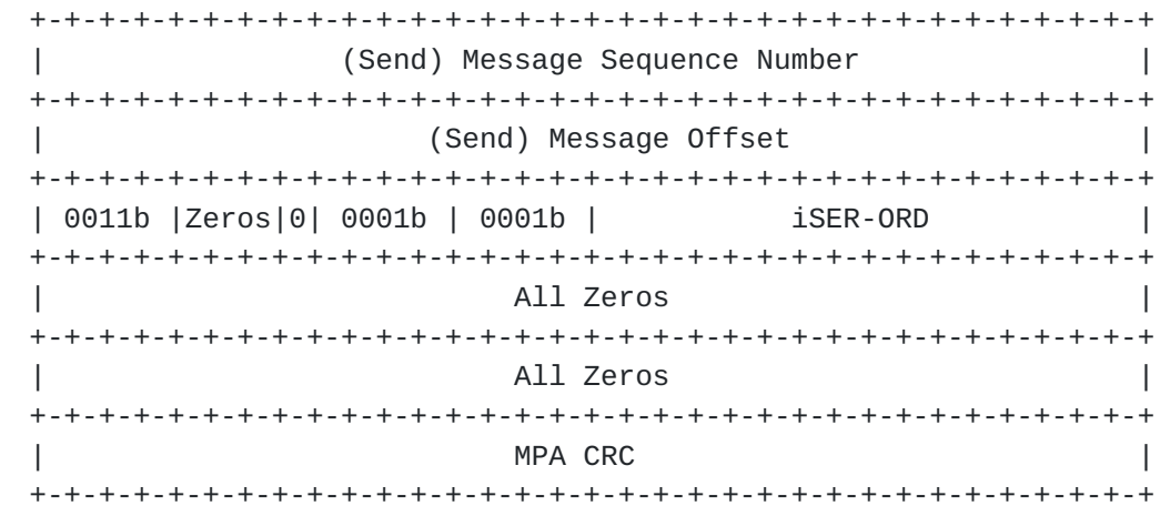
Figure 7 SendSE Message containing an iSER HelloReply Message
