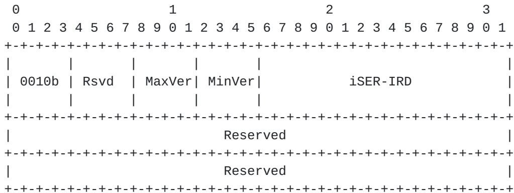
Figure 4 iSER Header Format for iSER Hello Message
