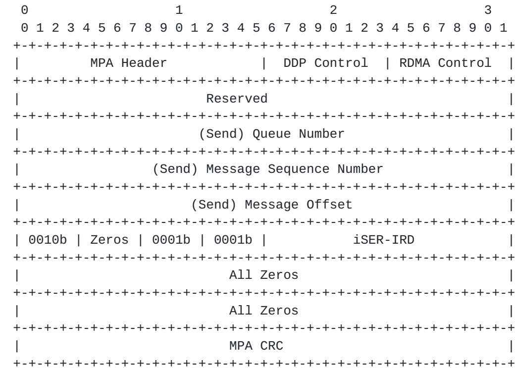
Figure 6 SendSE Message containing an iSER Hello Message
