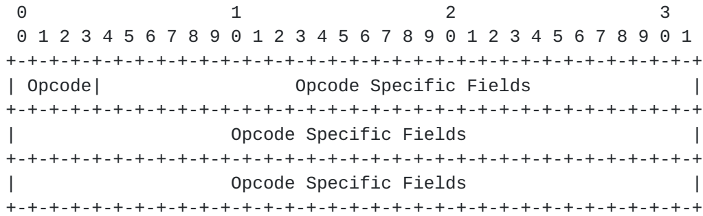
Figure 2 iSER Header Format
