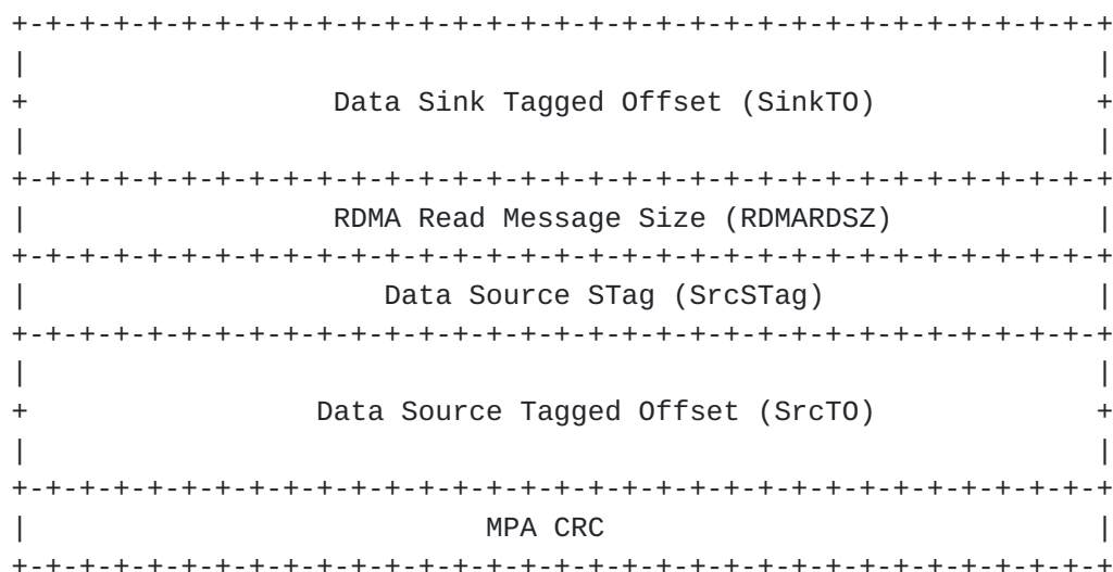
Figure 11 RDMA Read Request Message
