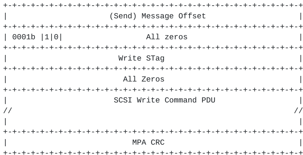
Figure 10 SendSE Message containing a SCSI Write Command PDU
