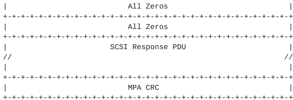
Figure 13 SendInvSE Message containing SCSI Response PDU
