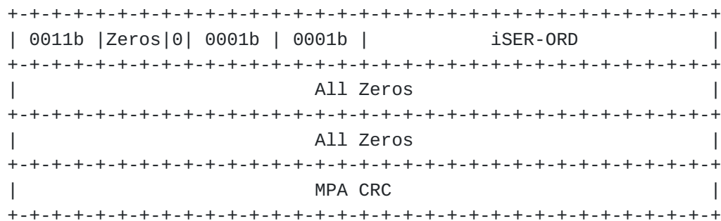
Figure 7 SendSE Message containing an iSER HelloReply Message
