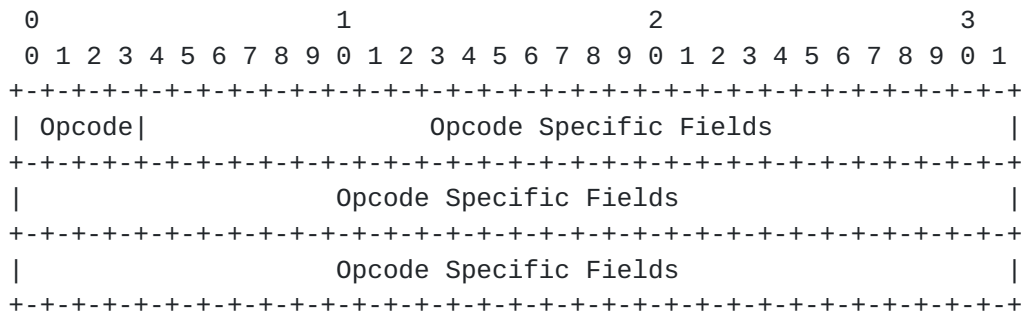
Figure 2 iSER Header Format
