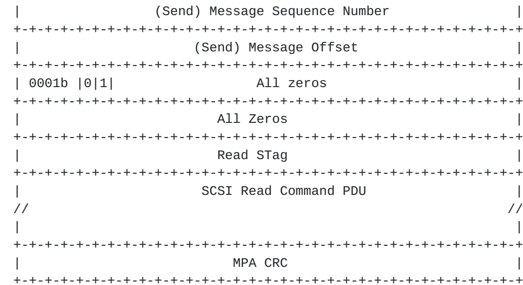
Figure 8 SendSE Message containing a SCSI Read Command PDU
