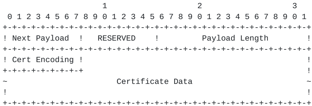
Figure 10: Certificate Payload Format
