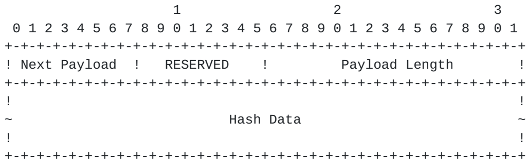
Figure 12: Hash Payload Format
