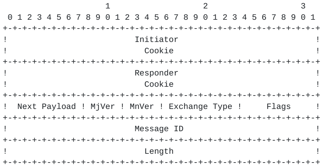
Figure 2: ISAKMP Header Format
