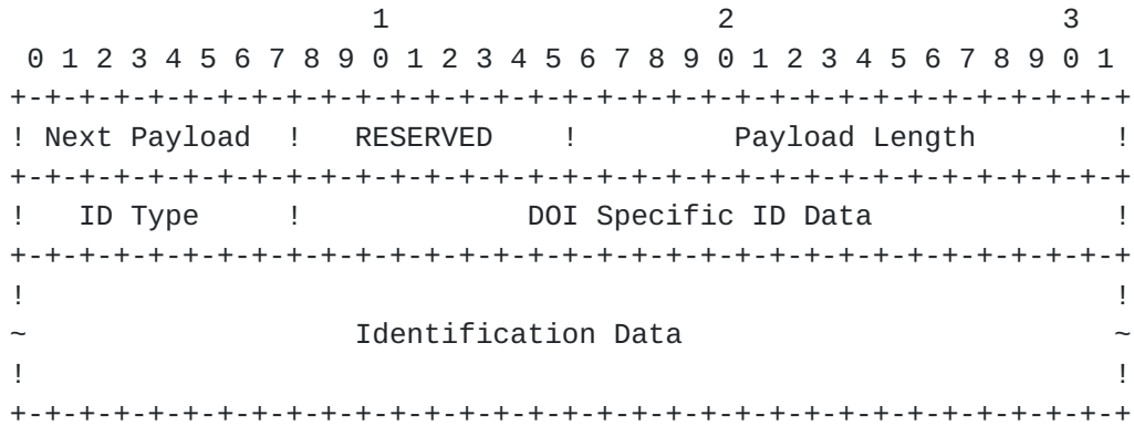
Figure 9: Identification Payload Format
