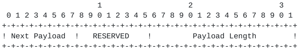
Figure 3: Generic Payload Header
