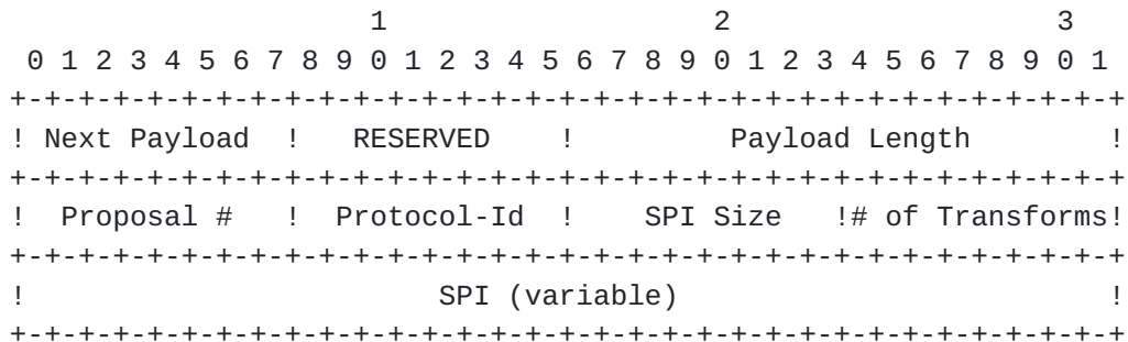
Figure 6: Proposal Payload Format
