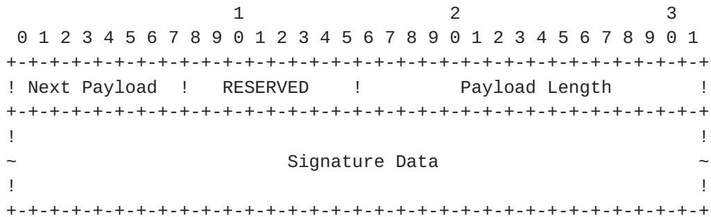
Figure 13: Signature Payload Format
