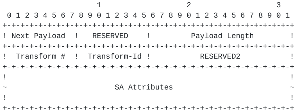
Figure 7: Transform Payload Format
