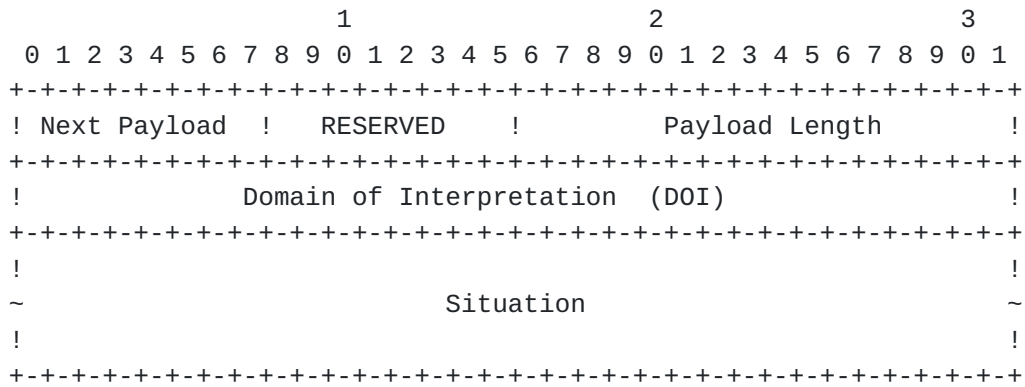
Figure 5: Security Association Payload
