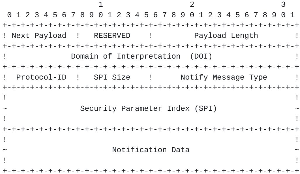
Figure 15: Notification Payload Format
