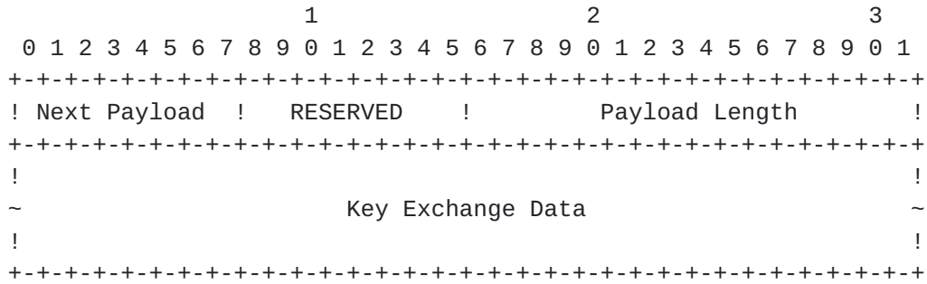
Figure 8: Key Exchange Payload Format
