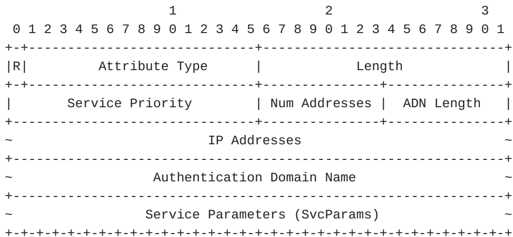
Figure 1: Attributes Format
