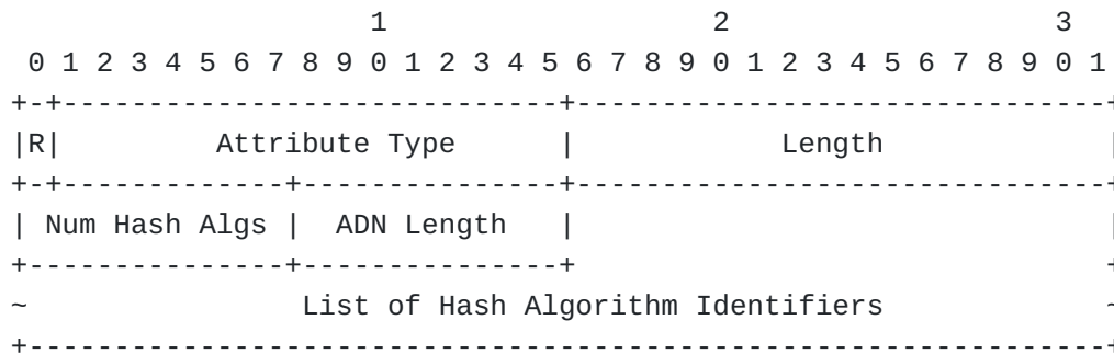
Figure 3: ENCDNS_DIGEST_INFO Attribute Format in CFG_REQUEST
