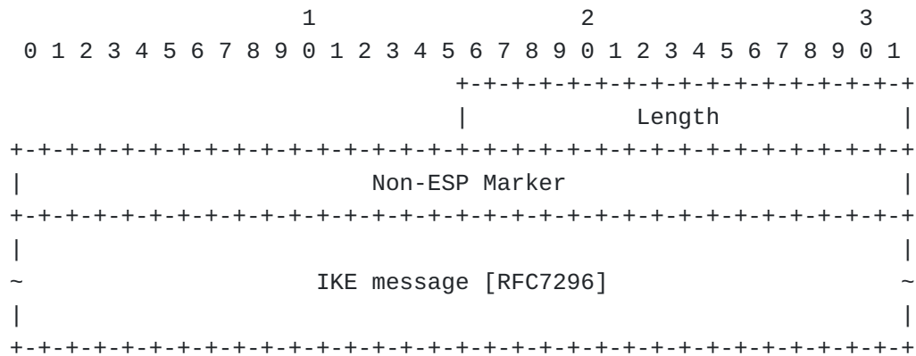
Figure 1: IKE message format for TCP encapsulation
