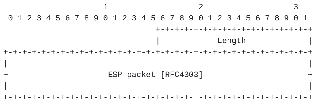
Figure 2: ESP packet format for TCP encapsulation
