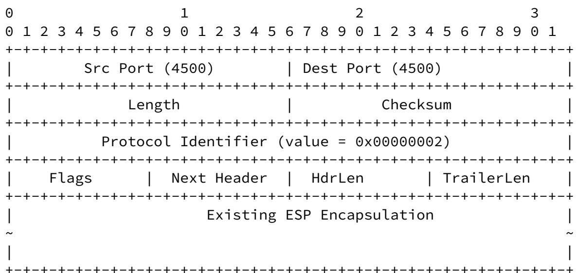
Figure 3 UDP-Encapsulated WESP Header
