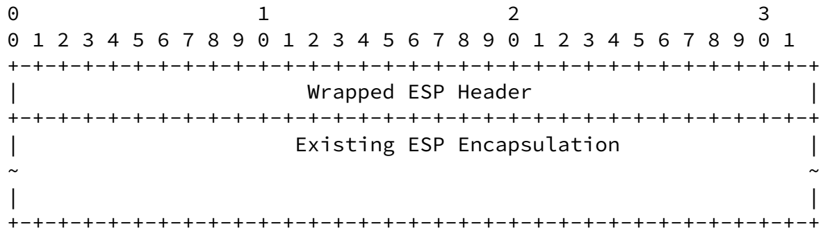
Figure 1 WESP Packet Format
