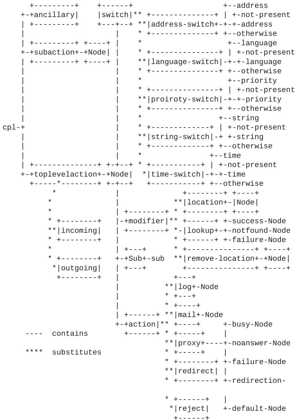
Figure 31: The structure of the XML schema for CPL
