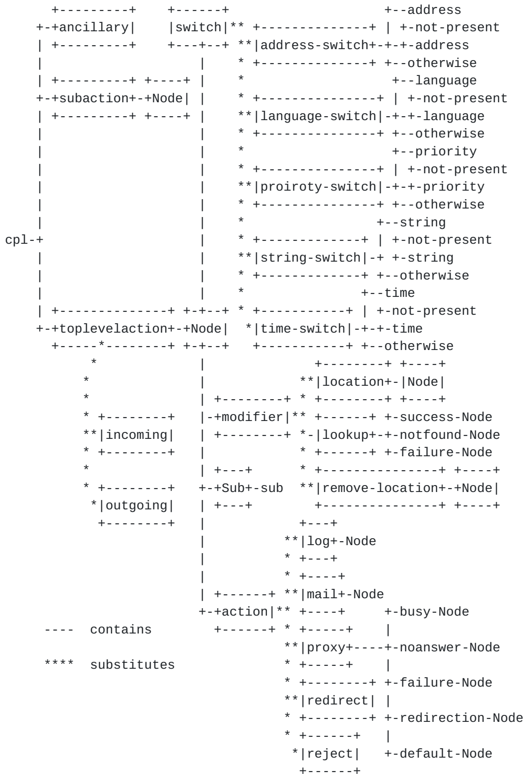
Figure 31: The structure of the XML schema for CPL
