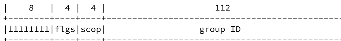
Figure 1: Generic IPv6 multicast address format
